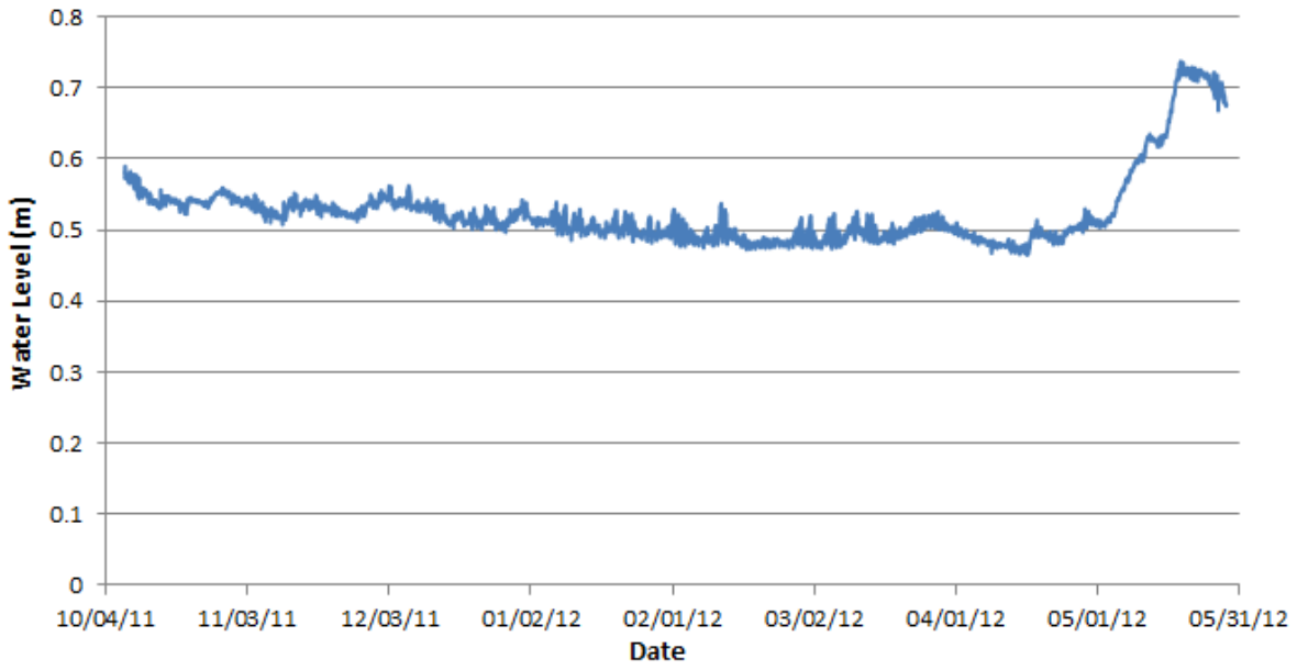
Figure 17C.12 Water Level at Station L2
