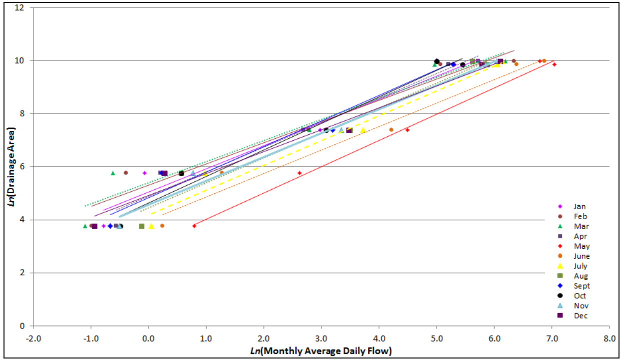
Figure 17D.3 Mean Monthly Average Daily Flows versus Drainage Areas Relationships
