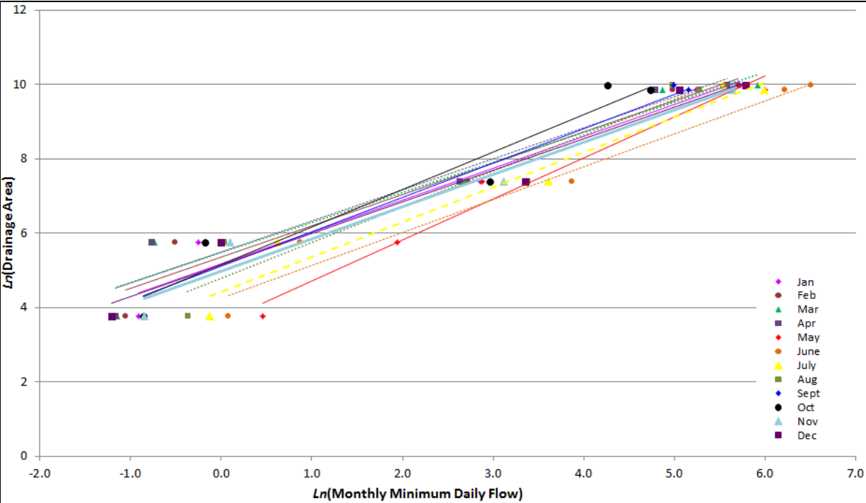
Figure 17D.2 Mean Monthly Minimum Daily Flows versus Drainage Areas Relationships
