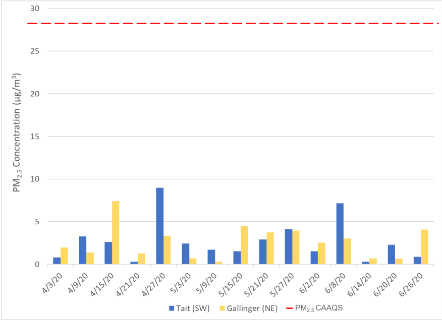
Figure 4-2: PM 2.5 Concentrations (Q2 2020)
