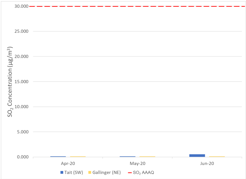
Figure 4-4: SO 2 Concentrations (Q2 2020)
