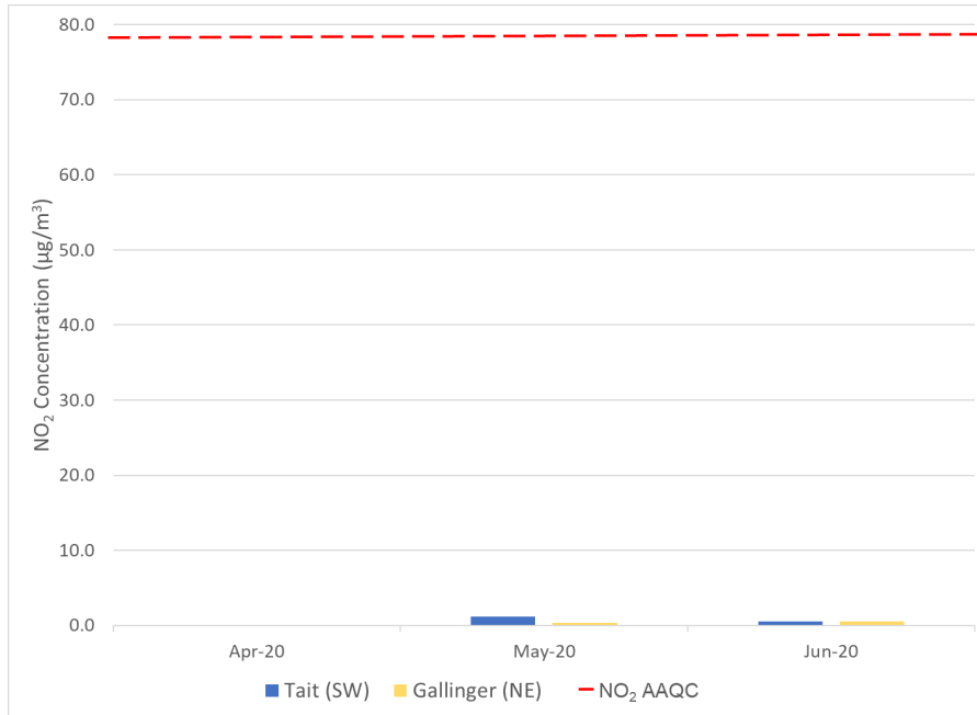
Figure 4-5: NO 2 Concentrations (Q2 2020)
