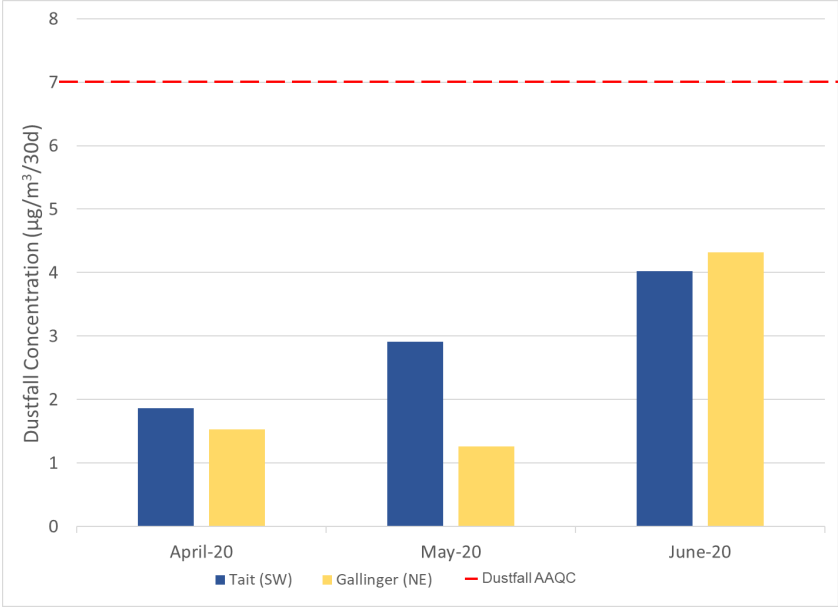
Figure 4-3: Dustfall Concentrations (Q2 2020)
