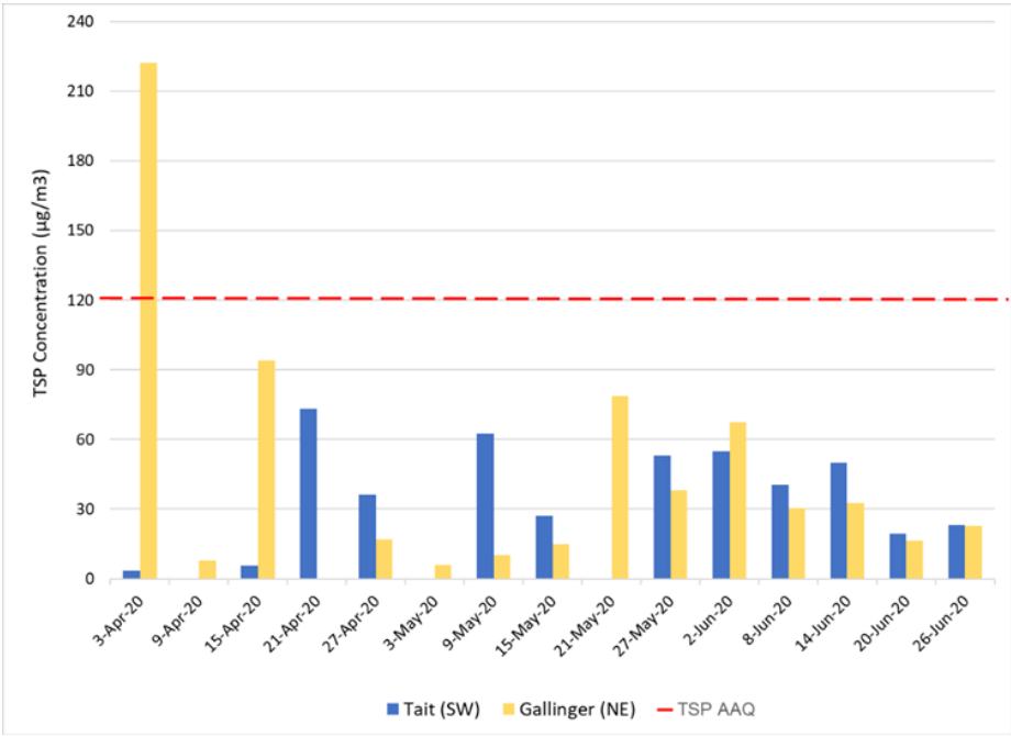
Figure 4-1: TSP Concentrations (Valid and Invalid Data) (Q2 2020)
