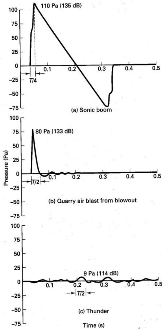
Figure 14-7 Comparison of air overpressure time history from 136 kg per delay quarry blast with thunder and sonic boom shows similarity in dominant period, T , and thus frequency, f (= 1/T) .
