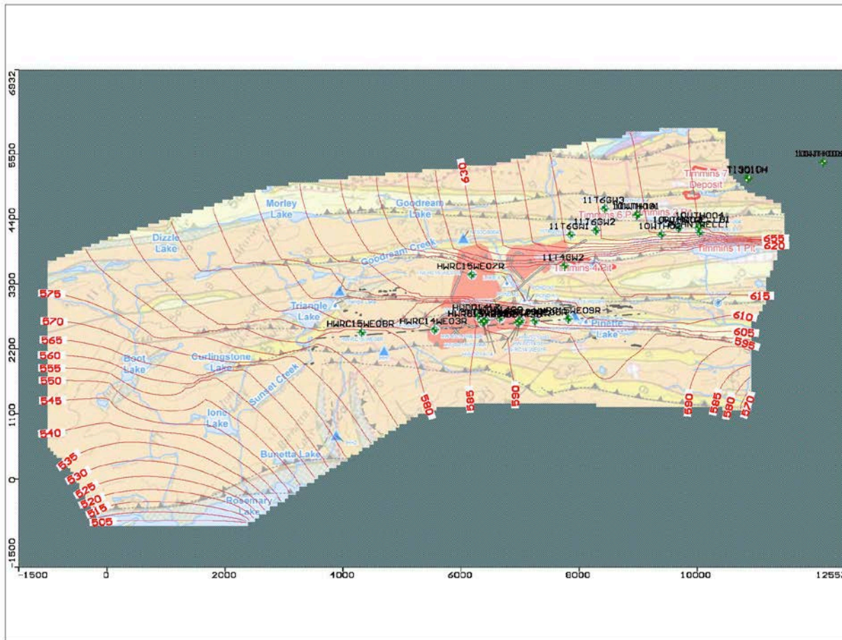
Figure 2-5 Piezometric Map at the end of Phase I of Pit Dewatering
