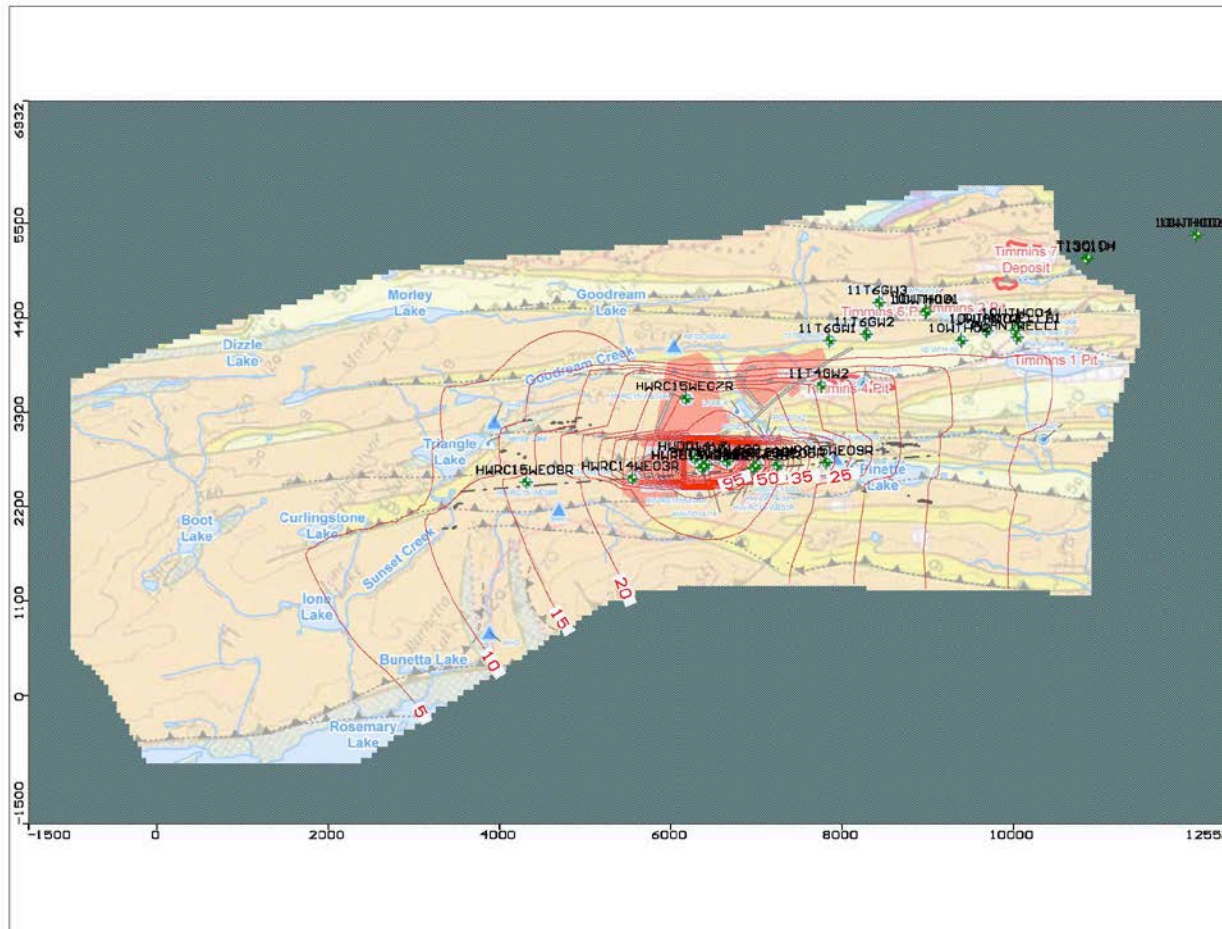
Figure 2-10 Groundwater Drawdown at the end of Phase III of Pit Dewatering
