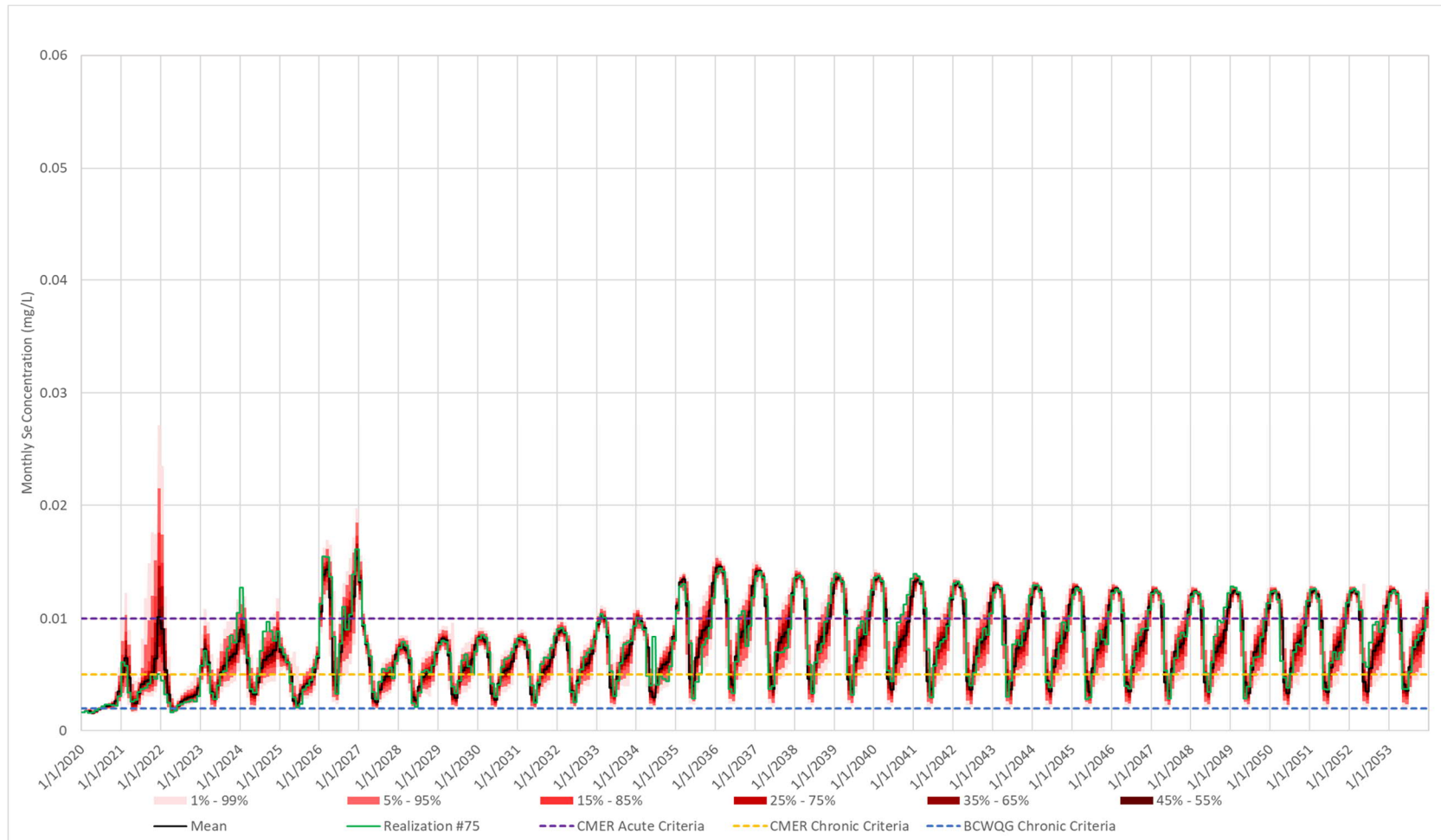
Figure 11.H-10: 95 th Percentile Selenium Predictions for Interim and Main Sediment Ponds
