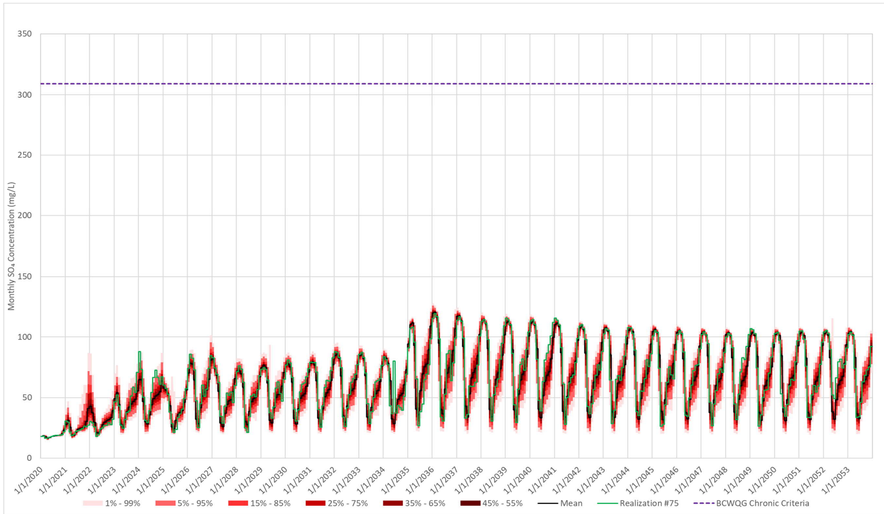
Figure 11.H-11: 50 th Percentile Sulphate Predictions for Interim and Main Sediment Ponds
