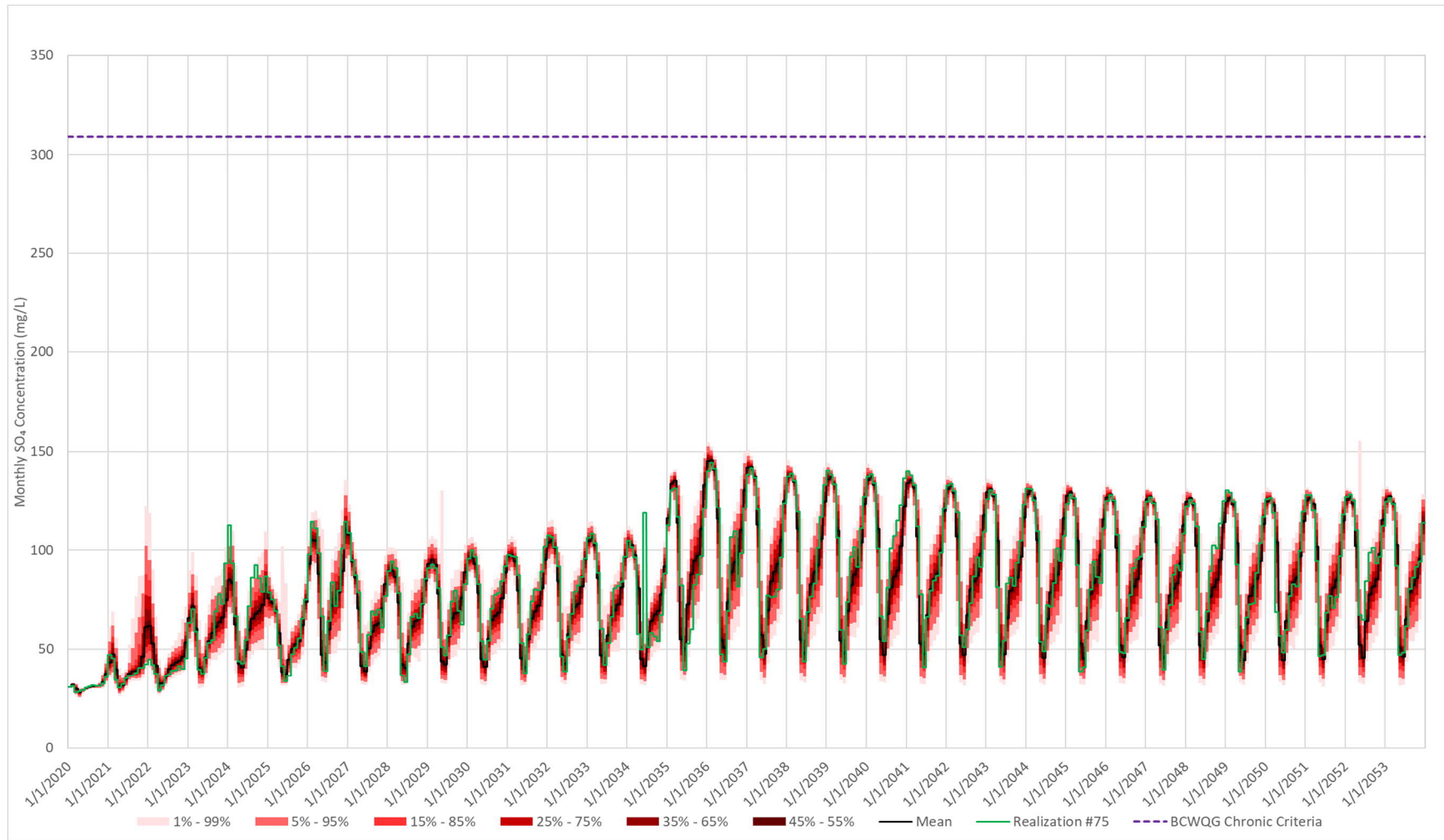
Figure 11.H-12: 95 th Percentile Sulphate Predictions for Interim and Main Sediment Ponds
