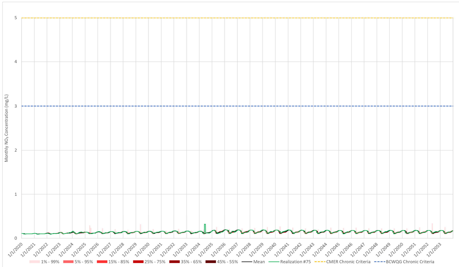
Figure 11.H-8: 95 th Percentile Nitrate Predictions for Interim and Main Sediment Ponds
