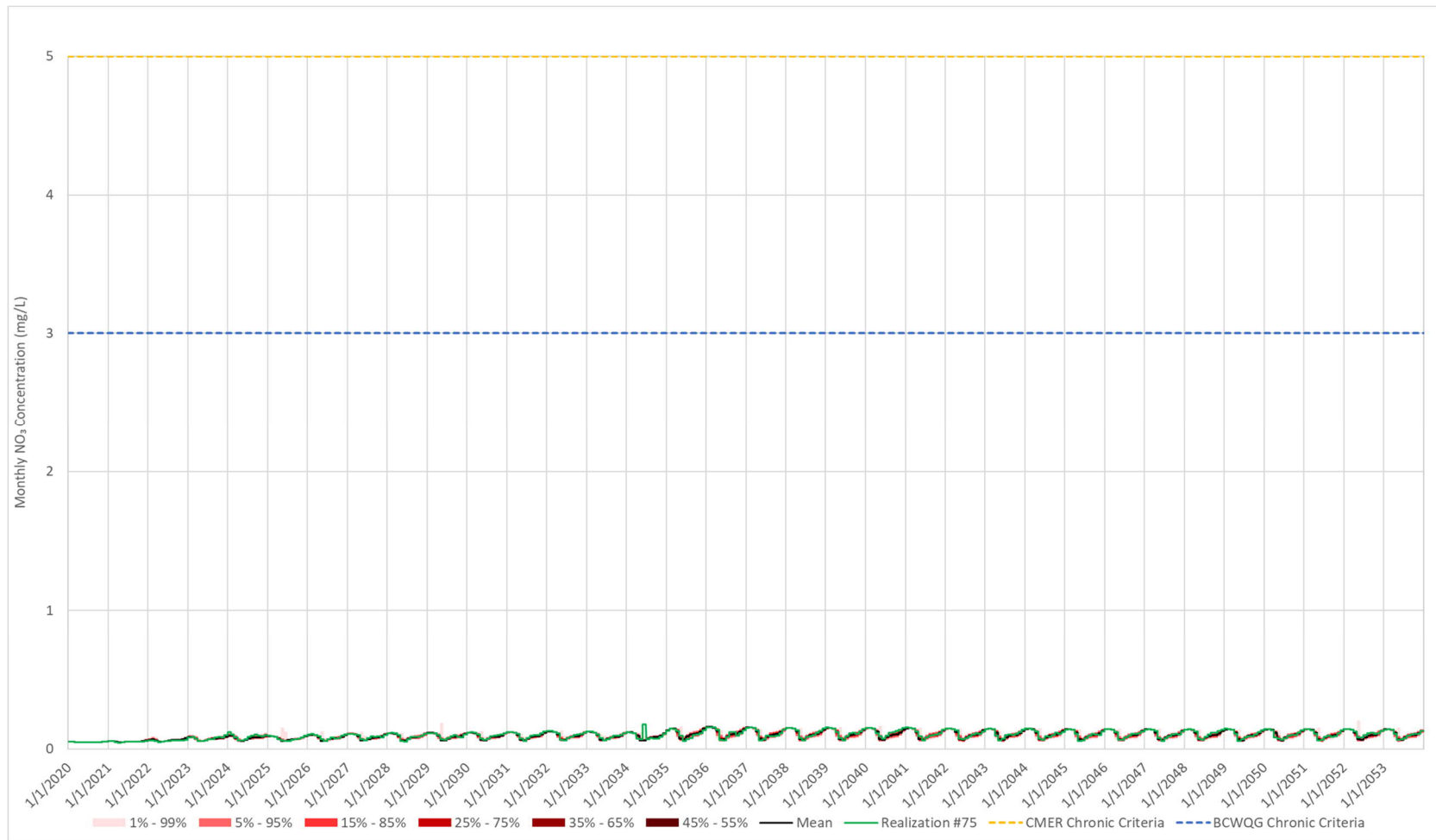
Figure 11.H-7: 50 th Percentile Nitrate Predictions for Interim and Main Sediment Ponds
