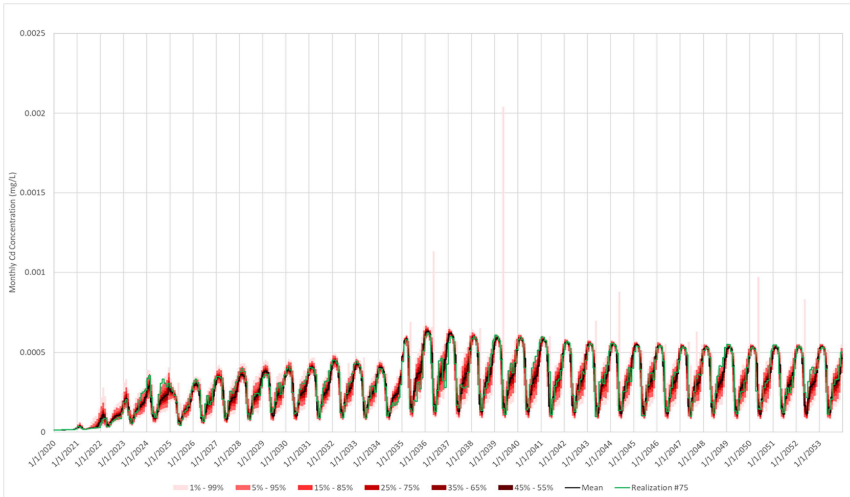
Figure 11.H-2: 95 th Percentile Cadmium Predictions for Interim and Main Sediment Ponds
