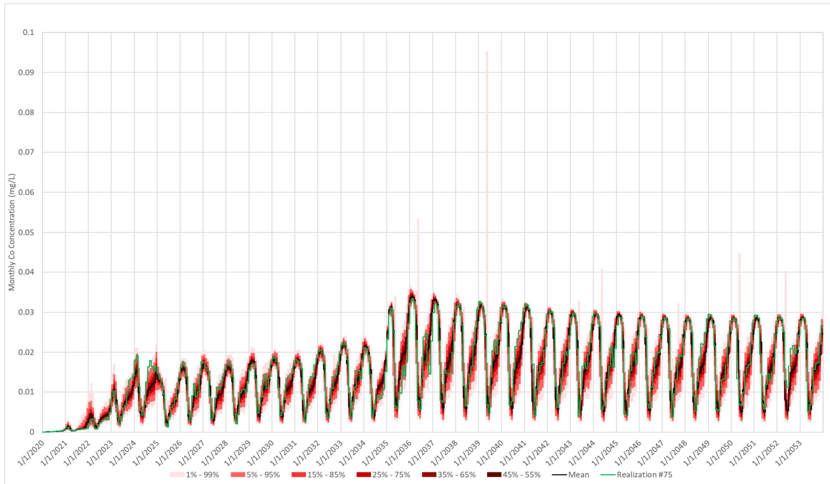
Figure 11.H-4: 95 th Percentile Cobalt Predictions for Interim and Main Sediment Ponds
