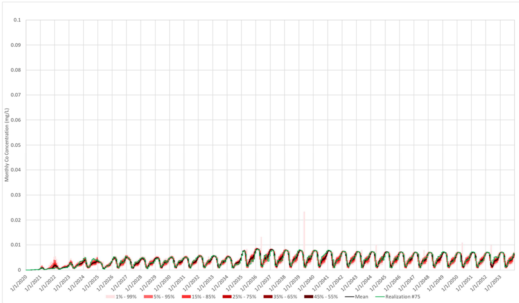
Figure 11.H-3: 50 th Percentile Cobalt Predictions for Interim and Main Sediment Ponds
