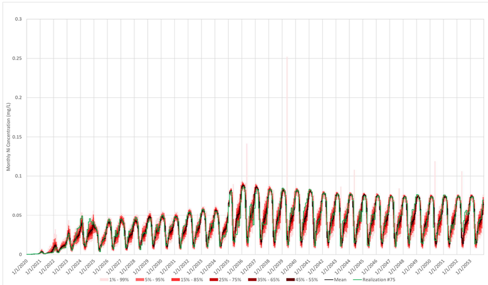
Figure 11.H-6: 95 th Percentile Nickel Predictions for Interim and Main Sediment Ponds
