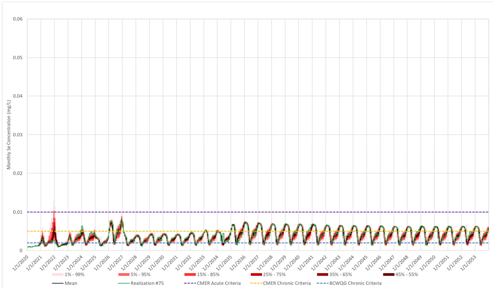
Figure 11.H-9: 50 th Percentile Selenium Predictions for Interim and Main Sediment Ponds
