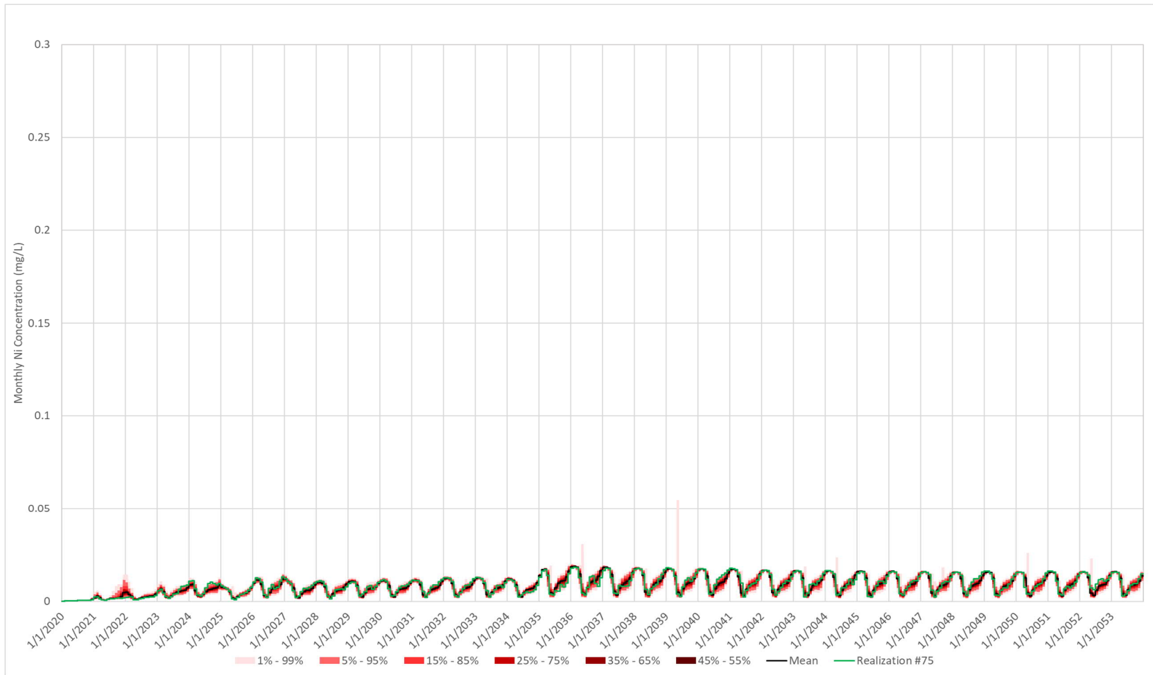
Figure 11.H-5: 50 th Percentile Nickel Predictions for Interim and Main Sediment Ponds
