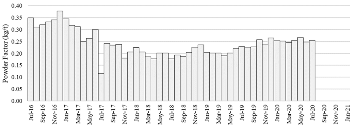
Figure 3: Monthly powder factor at Touquoy Mine from July 2016 to July 2020.
