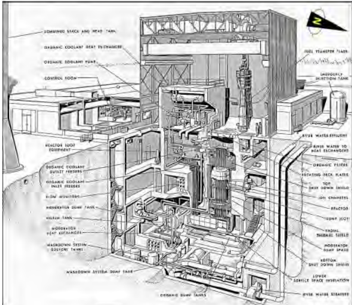
Figure 3-1: WR-1 Overview (CNL 2016a)
