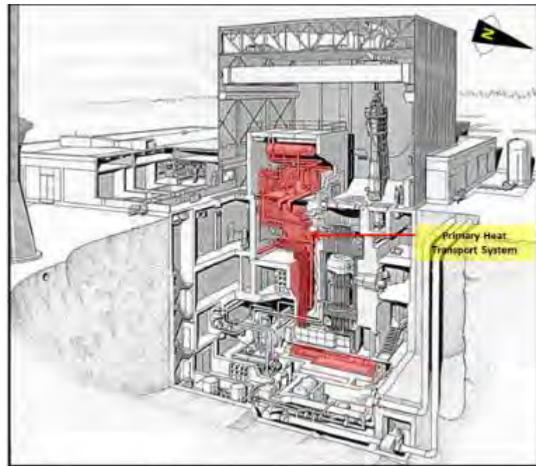
Figure 3-3: Primary Heat Transport System (CNL 2016a)
