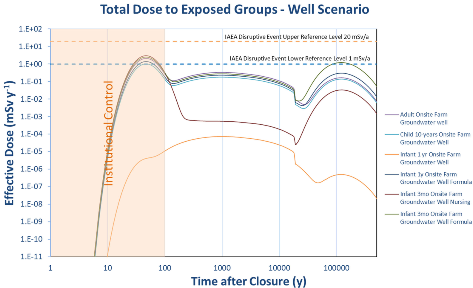
Figure D-1: Dose Rate to Human Receptors from Disruptive Events Scenario – Well in Plume
