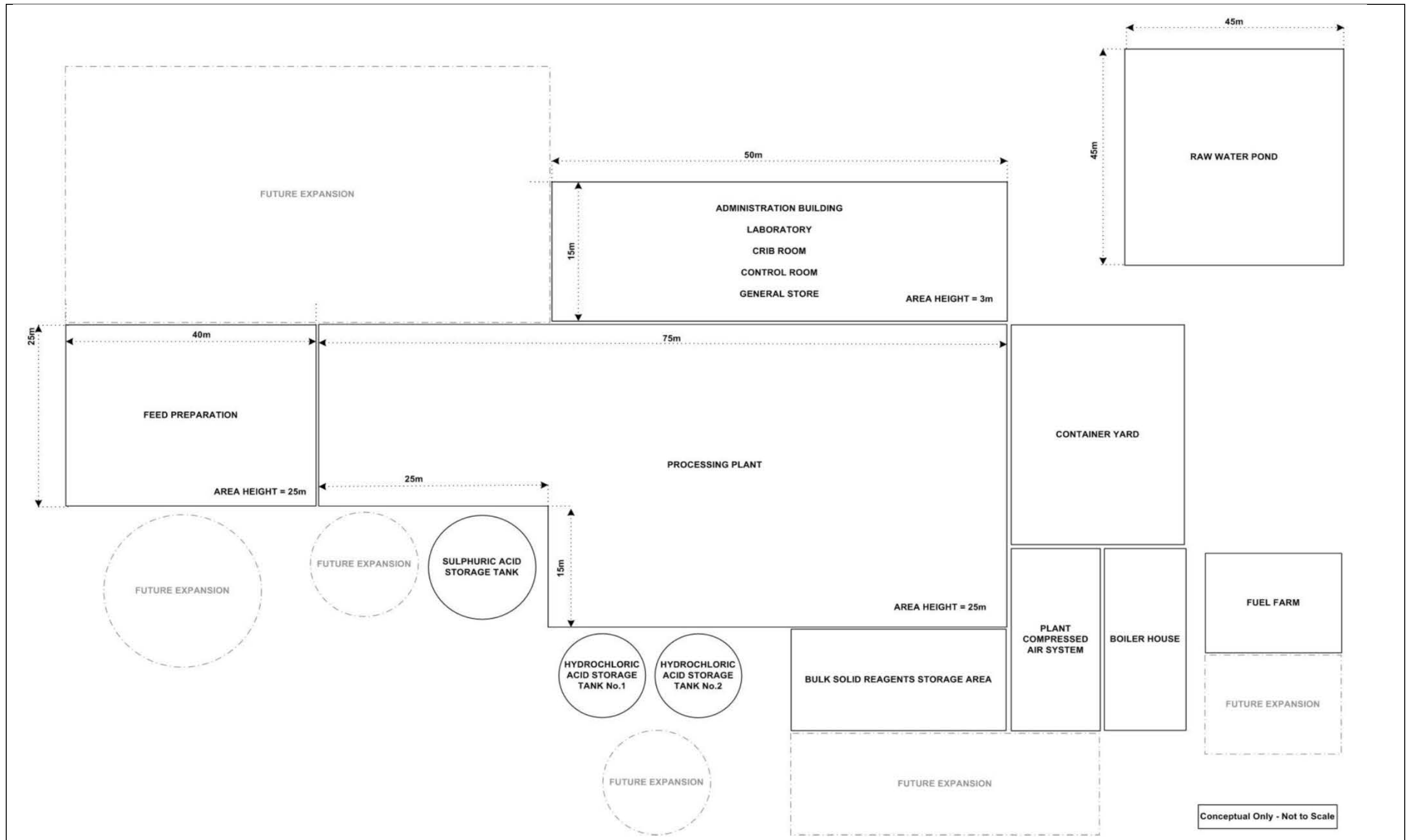
Figure 7 – Conceptual Processing Facility Layout
