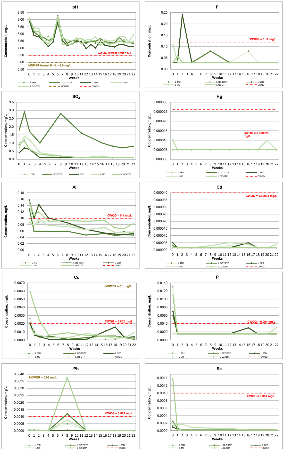
Figure C-1: Leprechaun Waste Rock Humidity Cell Plots
