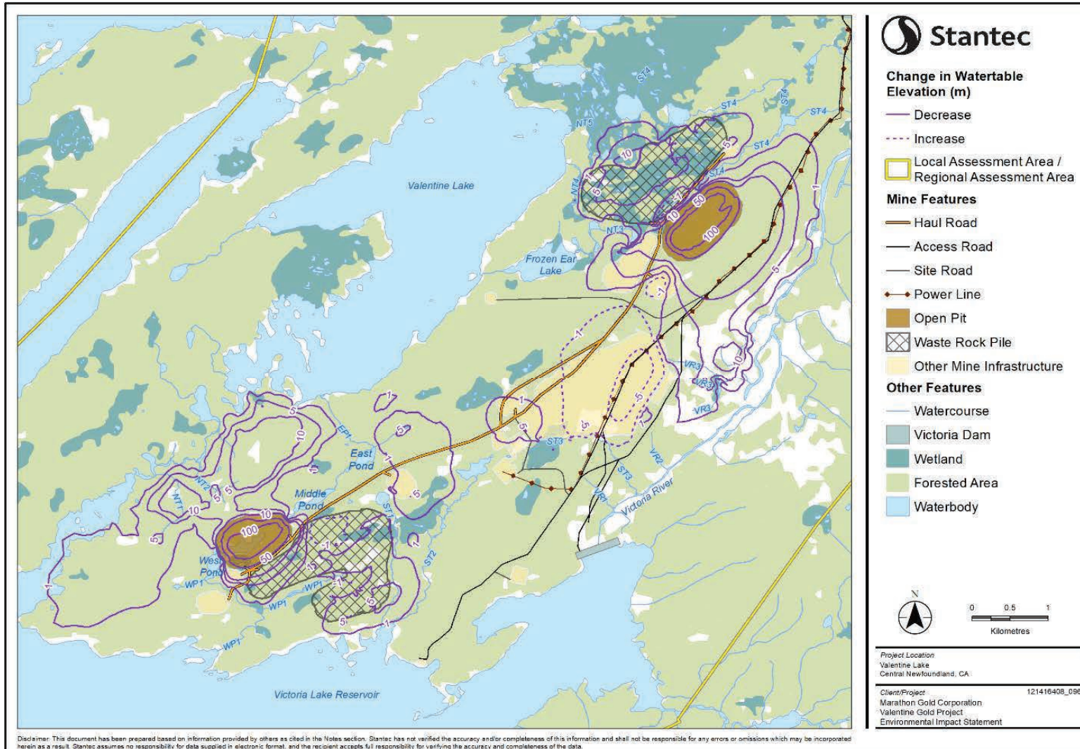
Figure 5-2 Change in Water Table Elevation at End of Project Operation
