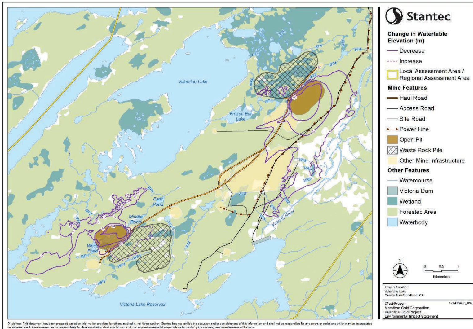
Figure 5-4 Change in Water Table Elevation Following Closure
