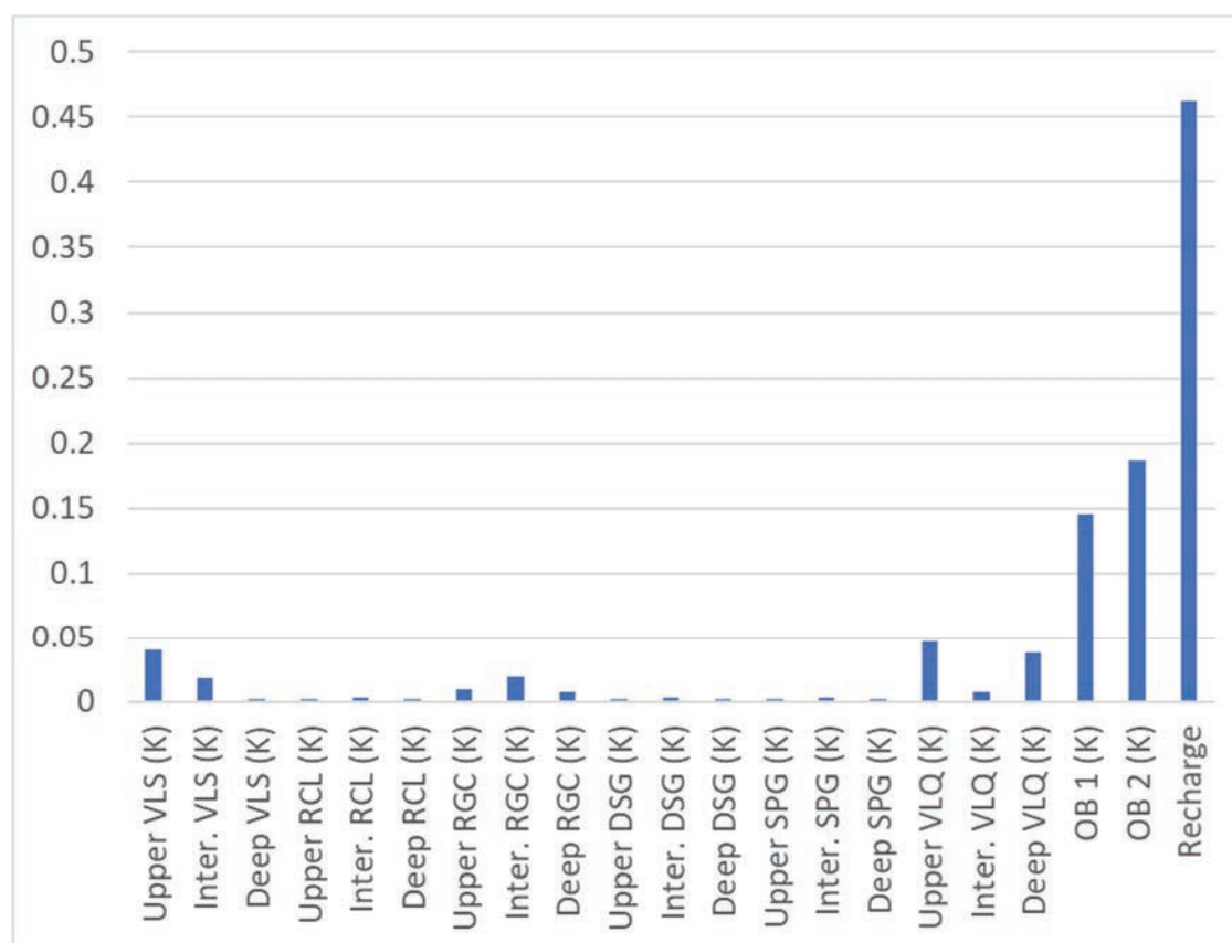
Figure 4-4 Relative Sensivities of Calibrated Parameters
