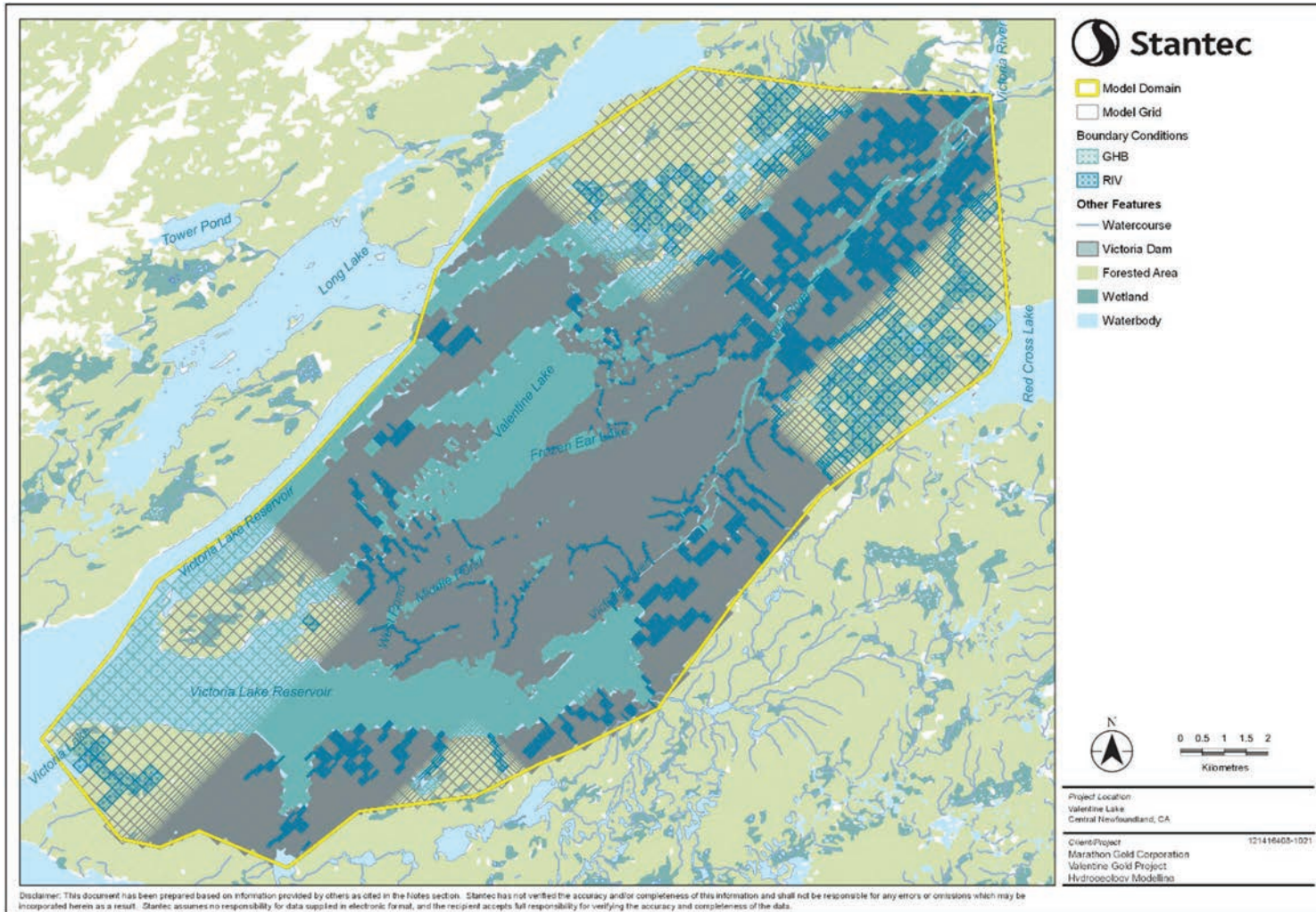
Figure 4-1 Model Domain and Boundary Conditions, showing location of General Head Boundary (GHB) and River (RIV)
