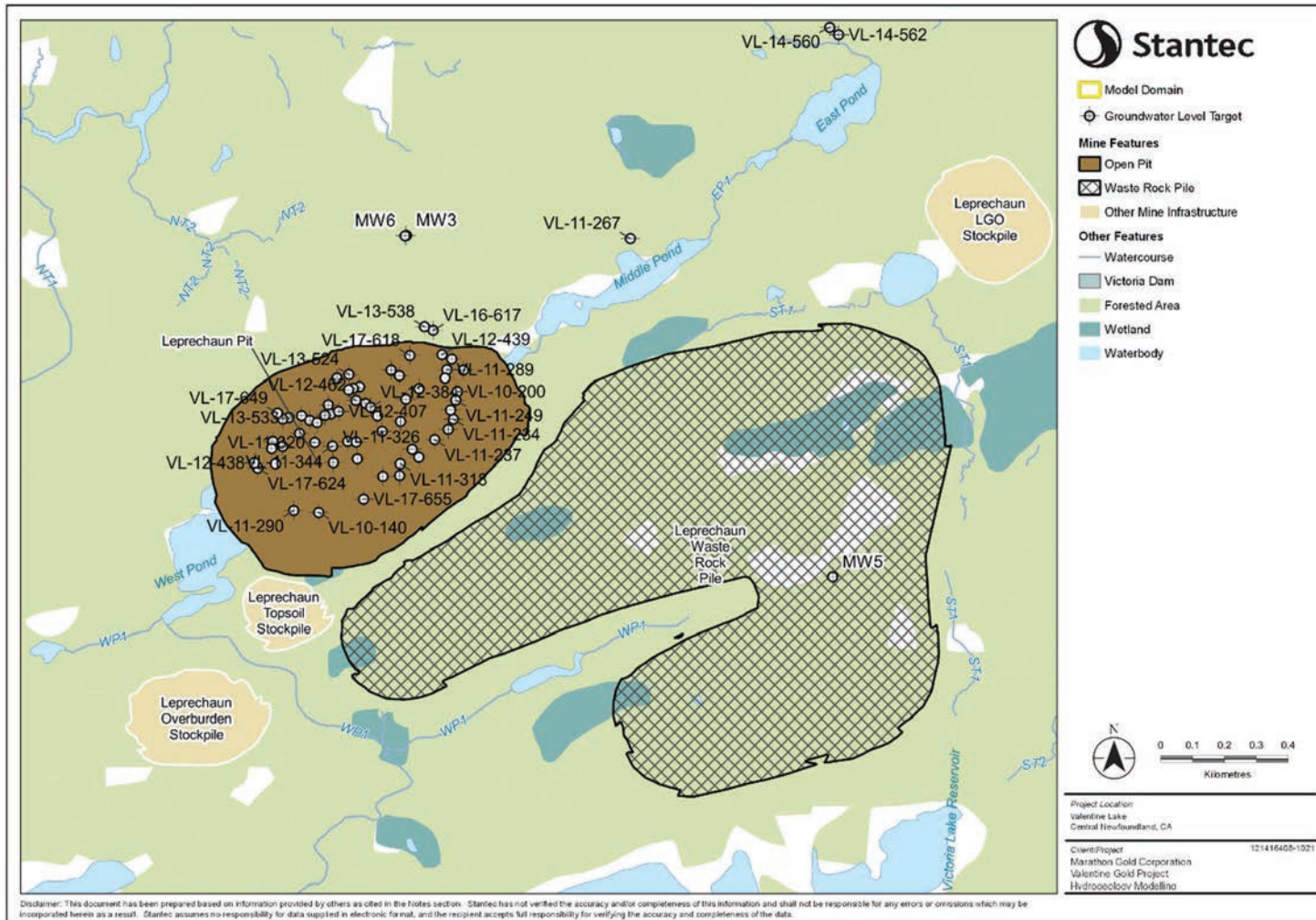
Figure 4-2a Groundwater Level Target Locations – Leprechaun Complex
