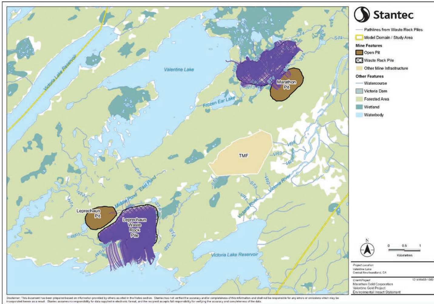
Figure 5-5 Particle Traces Illustrating Flow Paths from Waste Rock Piles and LGO Stockpiles at End of Project Operation
