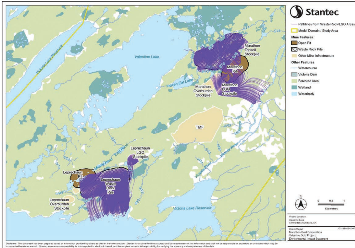
Figure 5-3 Particle Traces Illustrating Flow Paths from Waste Rock Piles and LGO Stockpiles at End of Project Operation
