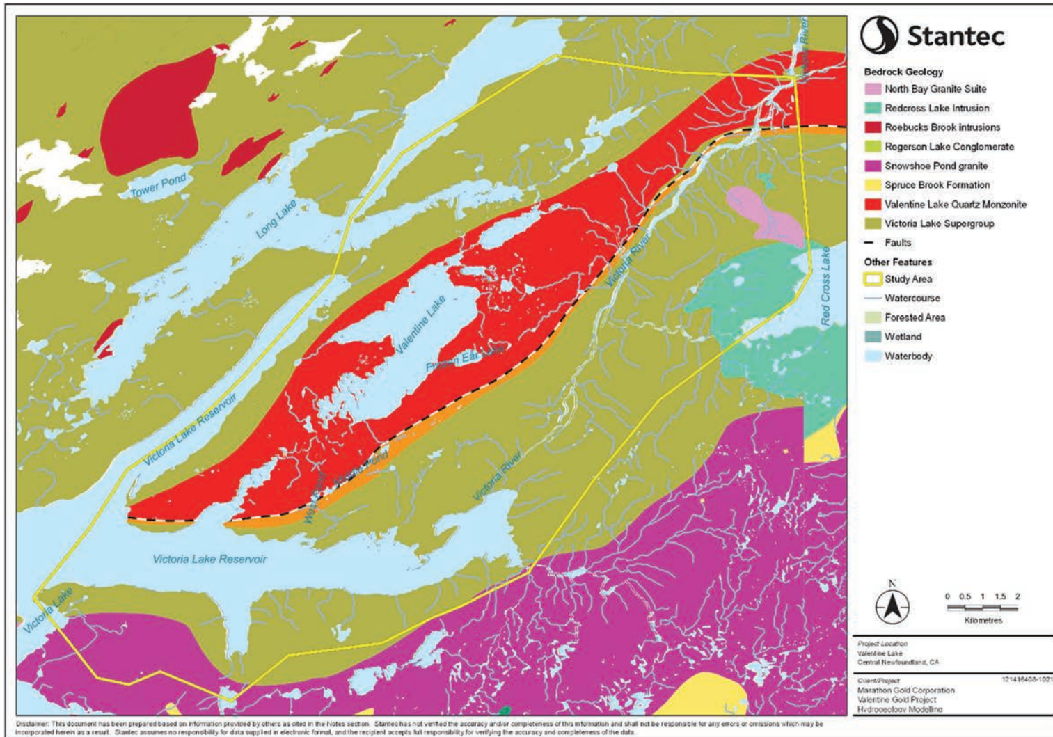
Figure 2-2 Bedrock Geology
