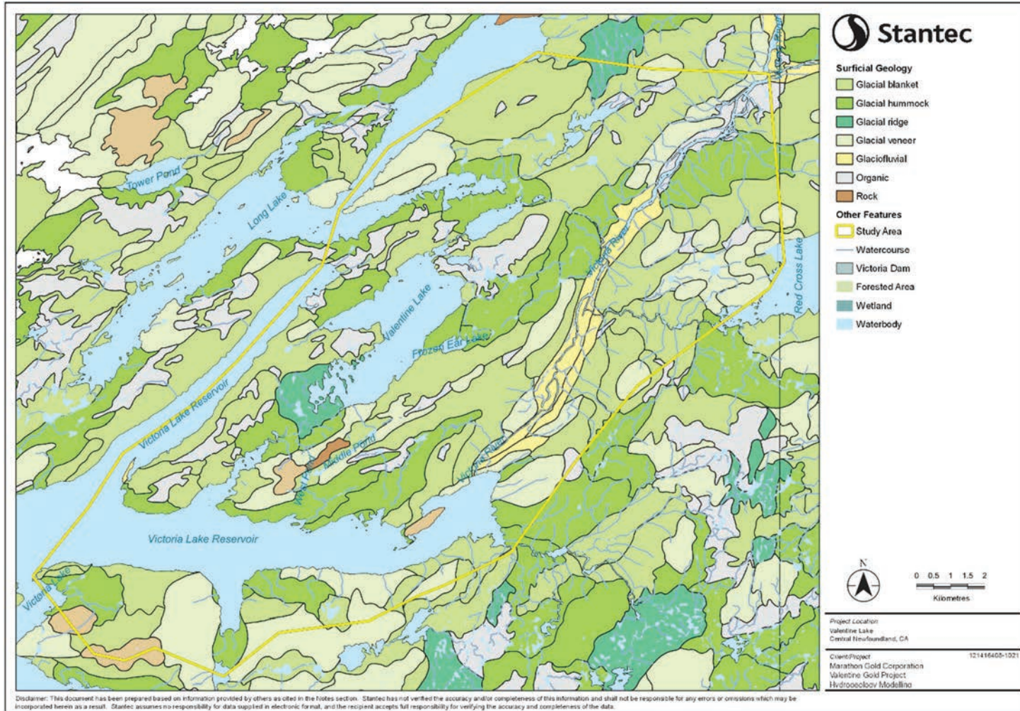
Figure 2-1 Surficial Geology
