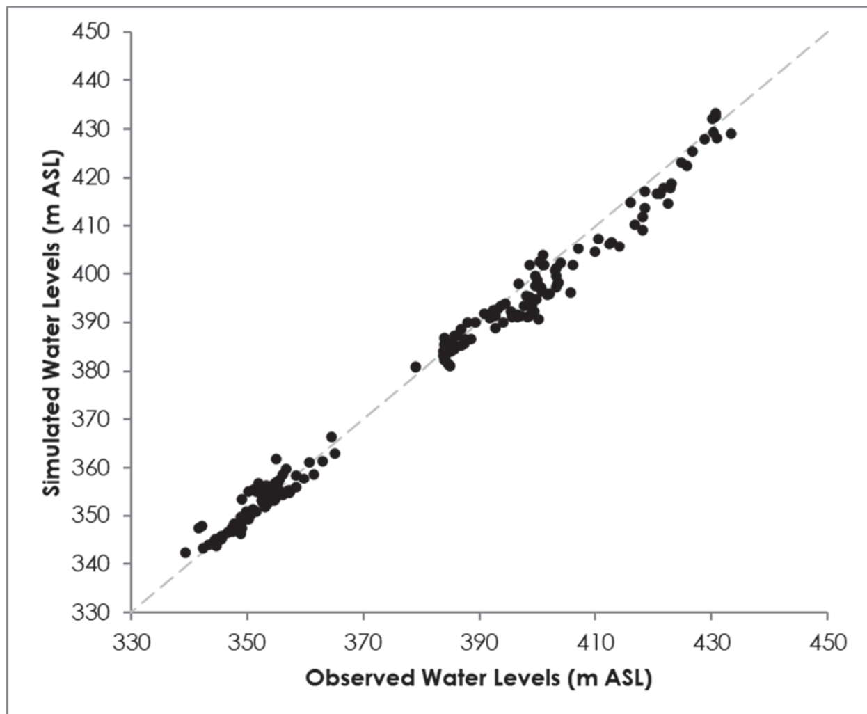
Figure 4-3 Comparison of Observed and Simulated Water Levels at end of Calibration
