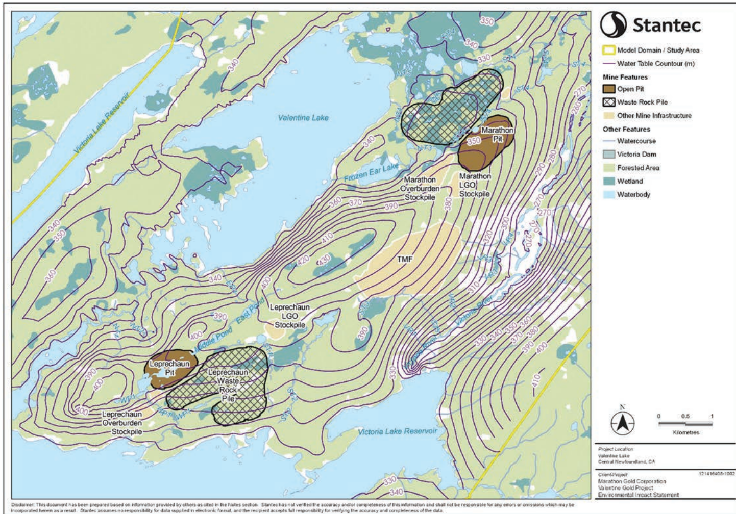
Figure 5-1 Baseline Water Table Elevation Contours
