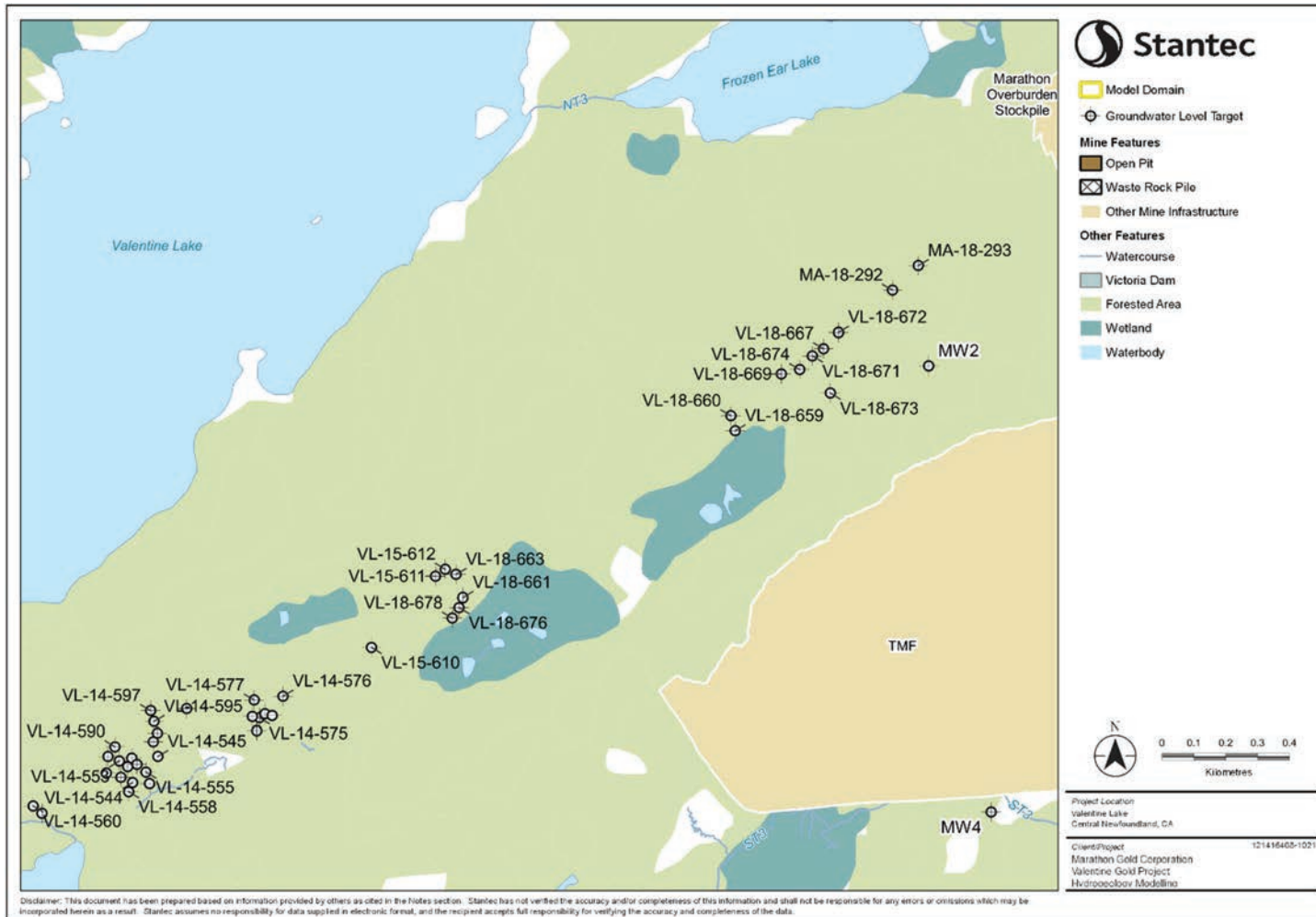
Figure 4-2b Groundwater Level Target Locations – Process Plant and TMF Complex
