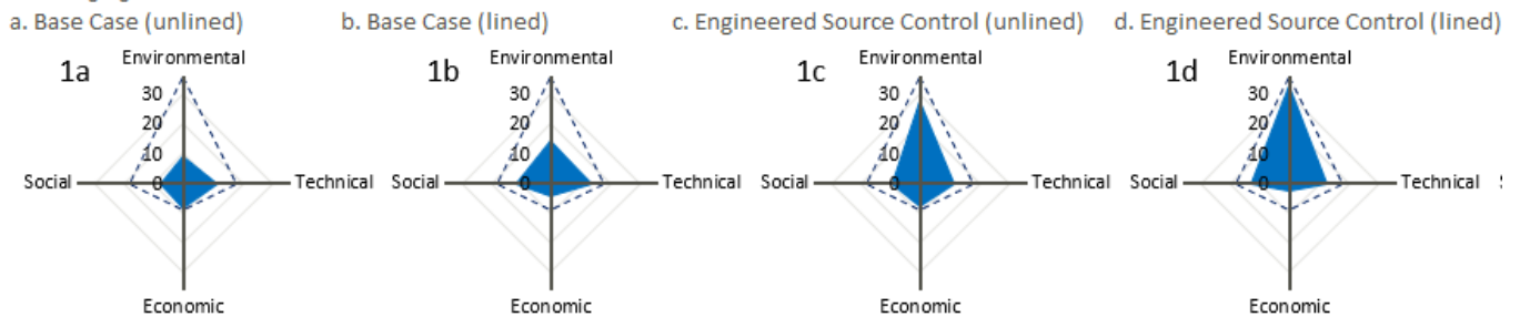
Figure 21: Radar Charts for the Waste Rock Multiple Accounts Analysis Results
