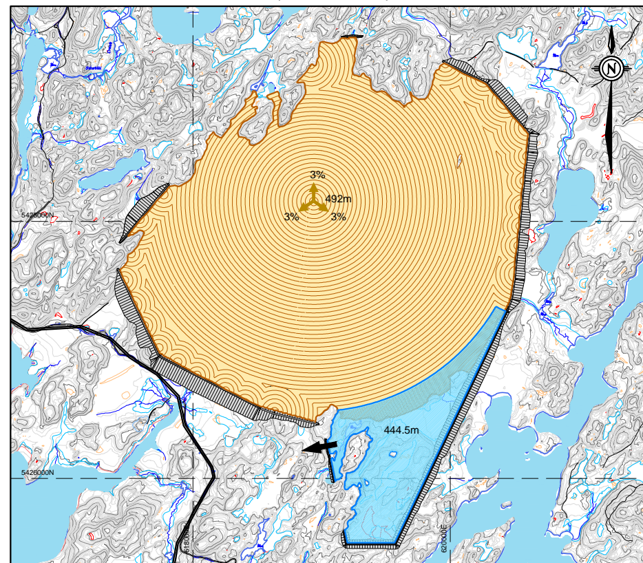
STAGE 4 (ULTIMATE) - YEAR 8 TO 10.5
