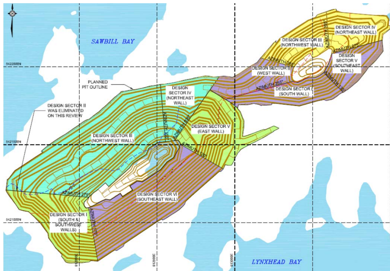
Figure 5-3: Pit Slope Design
