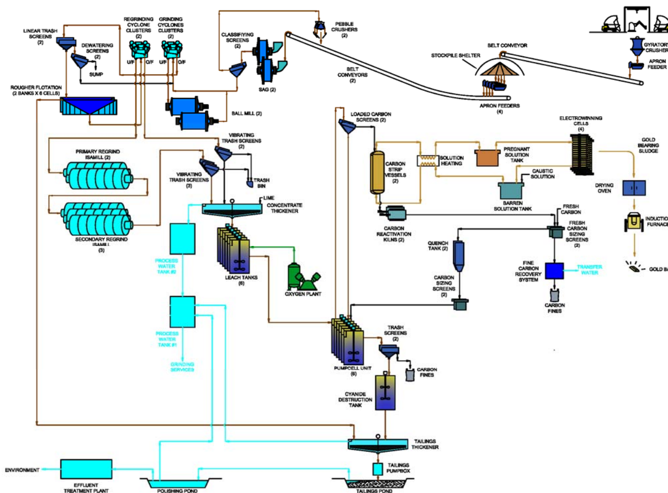
Figure 5-7: Simplified Process Overview
