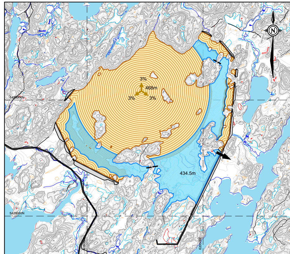
STAGE 1B (ROCKFILL) - YEAR 2.3 TO 3
