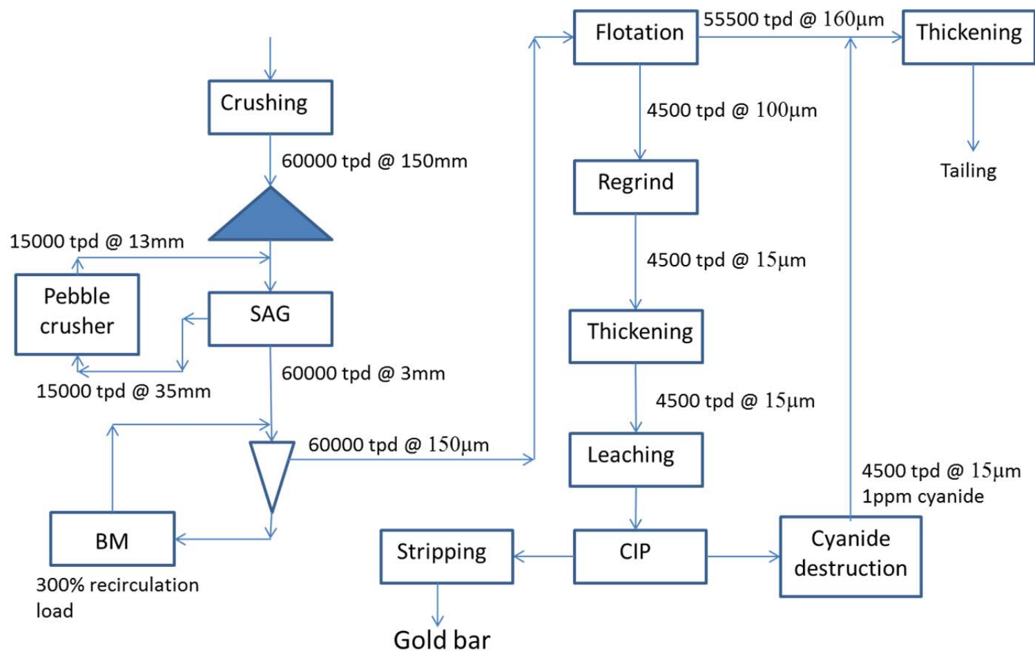
Figure 5-8: Process Flowsheet
