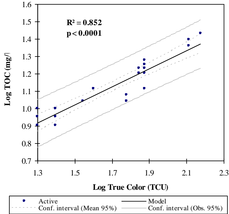
Figure 2H-42: Linear regression between total organic carbon (TOC) and true colour for data collected in the north arm of Stephens Lake: August 2005 and 2006
