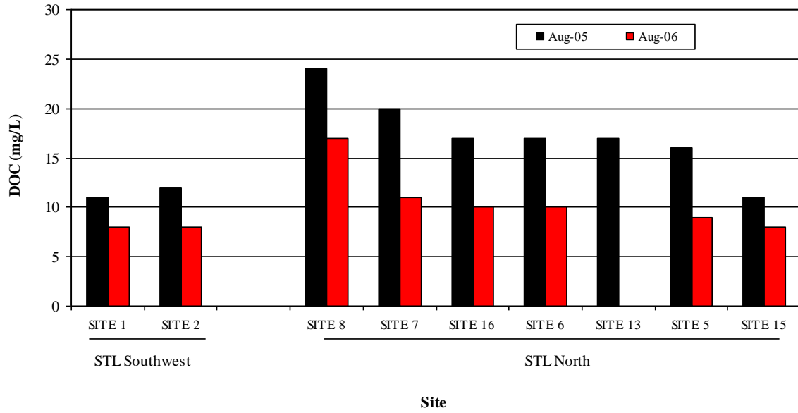
Figure 2H-38: Dissolved organic carbon (DOC) measured at sites located in the southwestern area of Stephens Lake (STL Southwest) and in the vicinity of O'Neil Bay (STL North). Sites in the north arm illustrated here represent a gradient from the nearshore area of O'Neil Bay out into the offshore area of the lake
