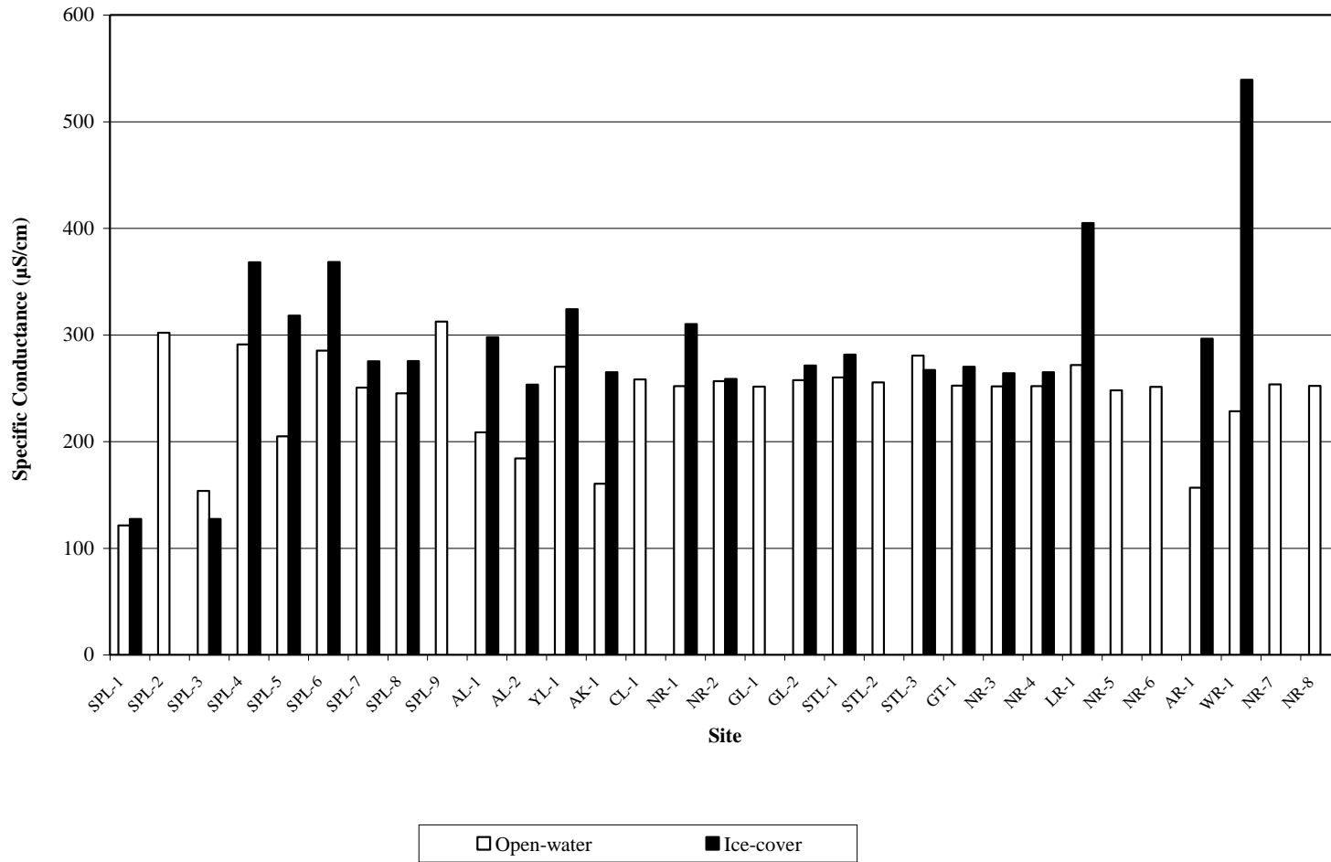
Figure 2H-18: Comparison of mean specific conductance ( in situ ) values measured in the open water and ice-cover seasons in the study area 2001–2007
