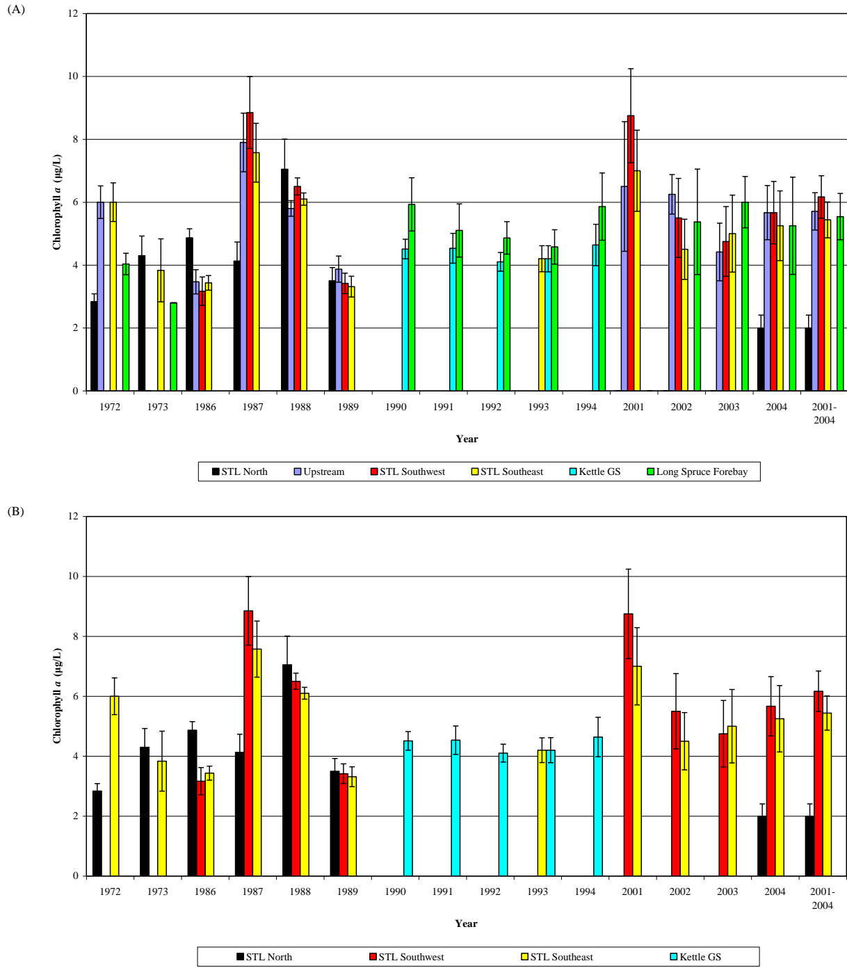
Figure 2E-7: Chlorophyll a (means ± standard error of the open water seasons) measured in Stephens Lake and upstream and downstream of the lake since 1972: (A) Stephens Lake and environs; and (B) Stephens Lake only
