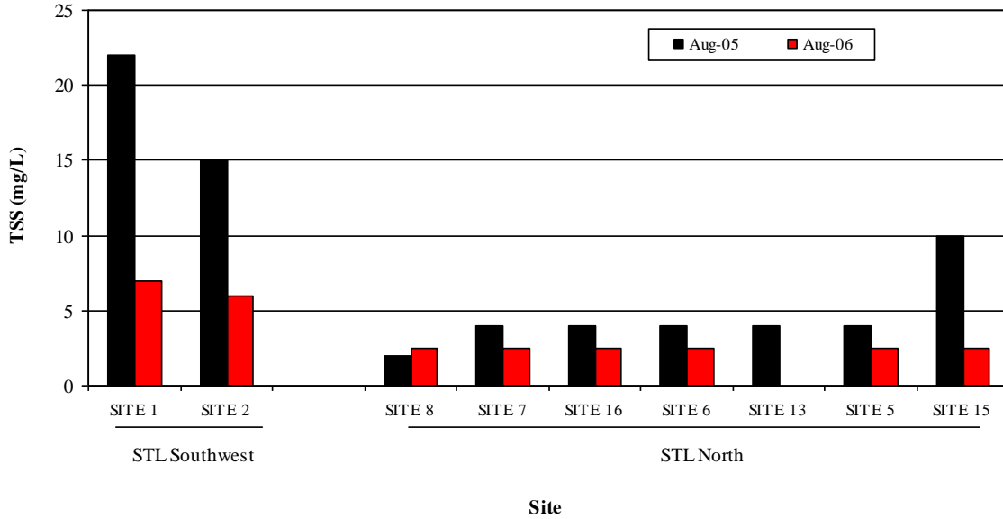
Figure 2H-28: Total suspended solids (TSS) measured at sites located in the southwestern area of Stephens Lake (STL Southwest) and in the vicinity of O'Neil Bay (STL North). Sites in the north arm illustrated here represent a gradient from the nearshore area of O'Neil Bay out into the offshore area of the lake
