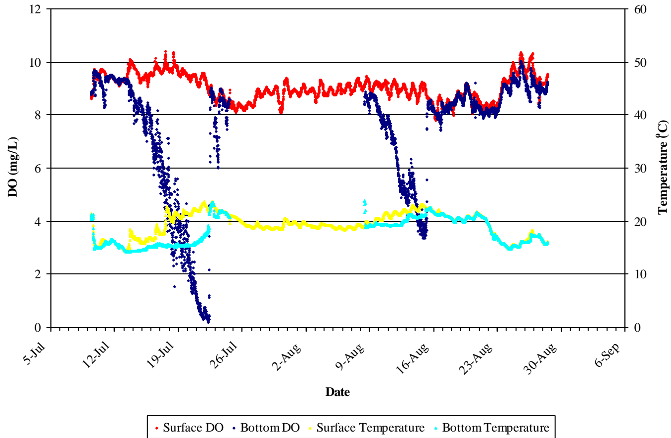
Figure 2H-24: Dissolved oxygen (DO) and temperature measured from loggers installed at Ross Wright Bay in Stephens Lake: summer 2008
