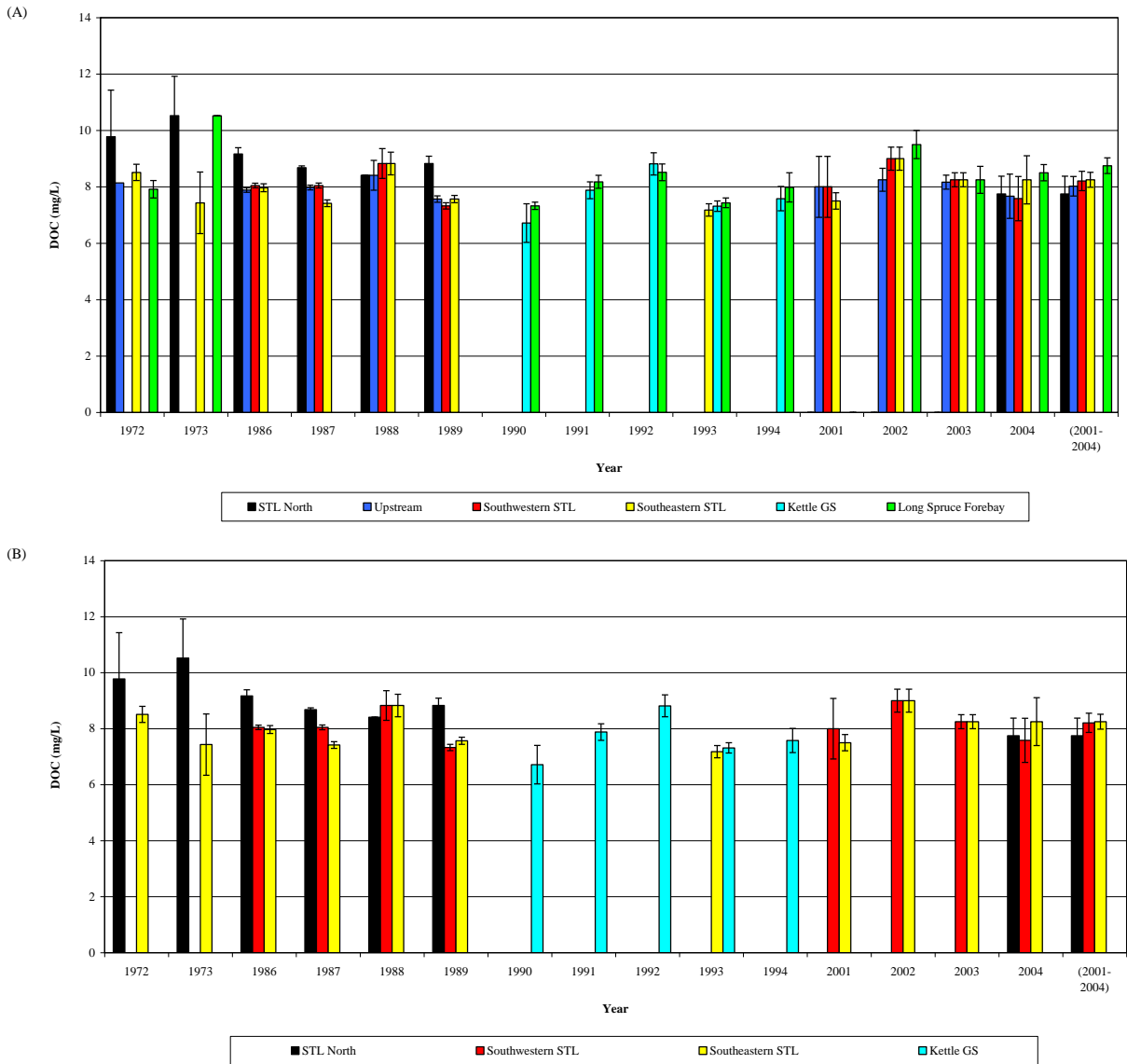
Figure 2E-4: Dissolved organic carbon (means \pm standard error of the open water seasons) measured in Stephens Lake and upstream and downstream of the lake since 1972: (A) Stephens Lake and environs; and (B) Stephens Lake only
