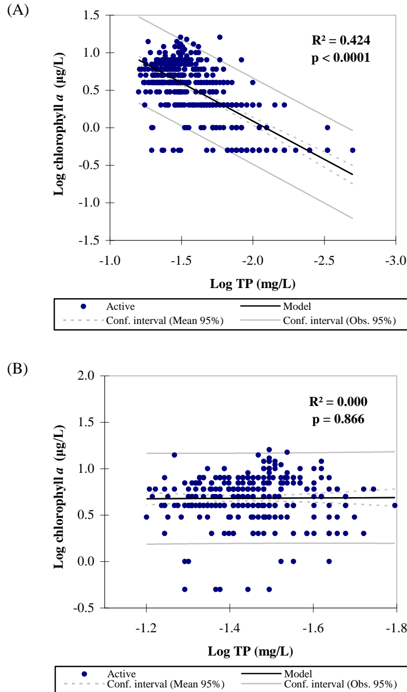
Figure 2H-9: Linear regression between total phosphorus (TP) and chlorophyll a measured (A) across the study area and (B) at mainstem sites only: open water seasons 1999–2004. Regressions should be interpreted with caution; data did not meet the assumptions of normality
