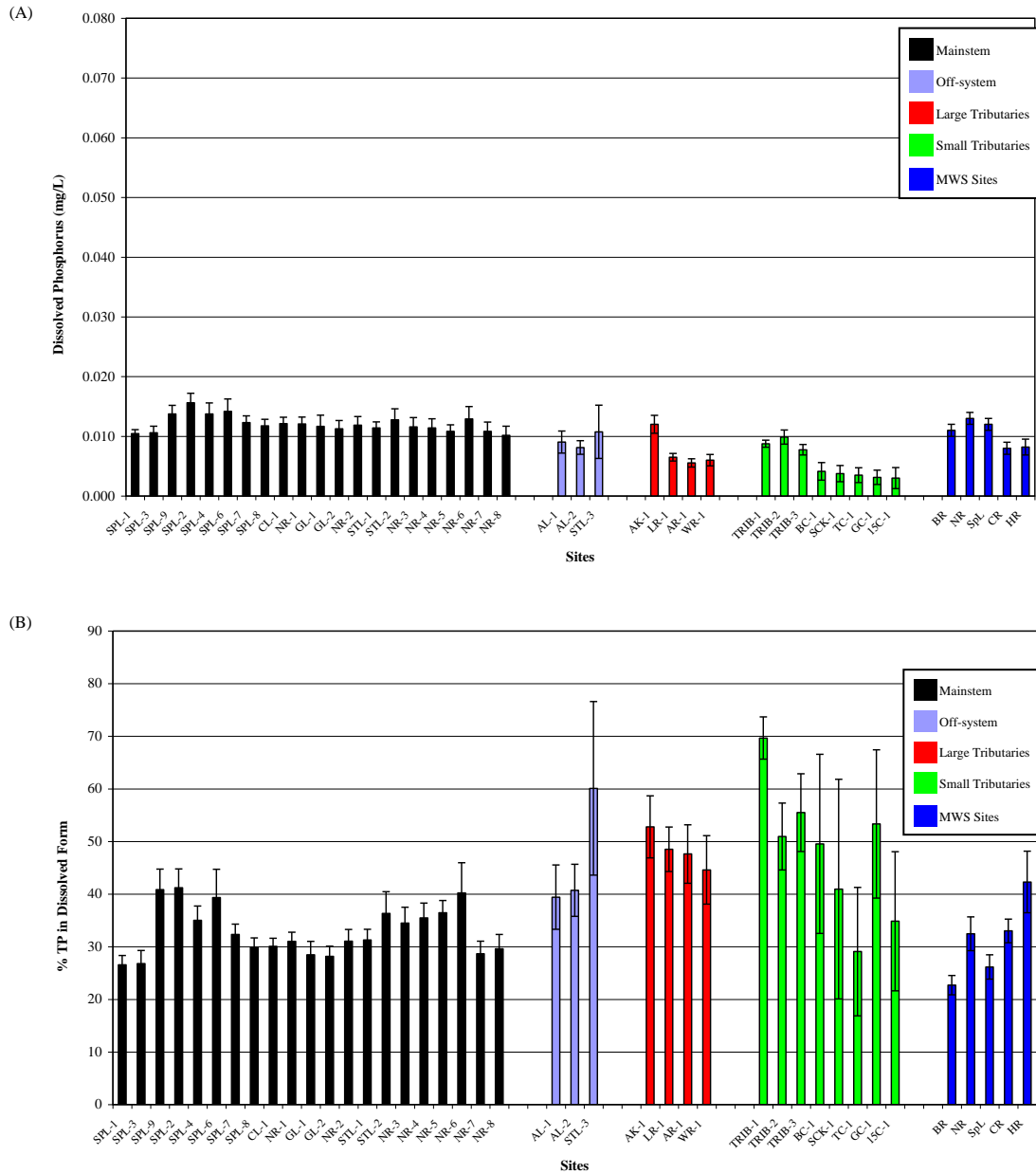
Figure 2-8: Open water season mean ( \pm standard error) (A) concentrations of total dissolved phosphorus and (B) percent total phosphorus (TP) in dissolved form measured at sites located on the mainstem of the lower Nelson River, off-system sites, large tributaries, small tributaries, and Manitoba Water Stewardship (MWS) monitoring sites in the Burntwood River (BR) at Thompson, the Nelson River (NR) at Sipiweesk Lake, the Churchill River (CR) and at Granville Lake (GL), and the historical Environment Canada site on the Hayes River (HR) at God’s River. Means for MWS sites represent the period of 1997–2006 and the mean for the Hayes River represents the period of 1993–1995
