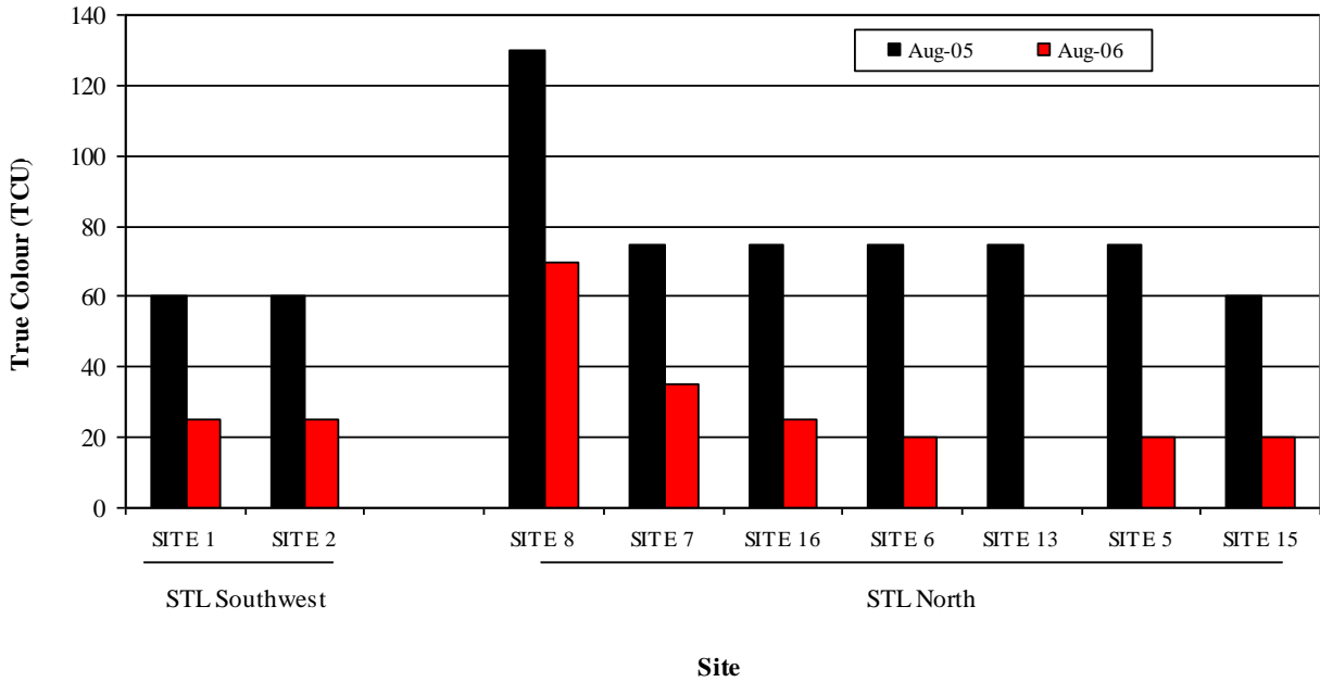
Figure 2H-30: True colour measured at sites located in the southwestern area of Stephens Lake (STL Southwest) and in the vicinity of O'Neil Bay (STL North). Sites in the north arm illustrated here represent a gradient from the nearshore area of O'Neil Bay out into the offshore area of the lake
