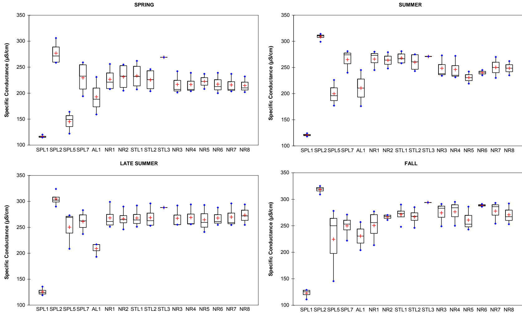
Figure 2H-6: Specific conductance ( in situ ) box plots for data collected from Split Lake to Gillam Island in the open water seasons 2001–2004. Data represent surface measurements
