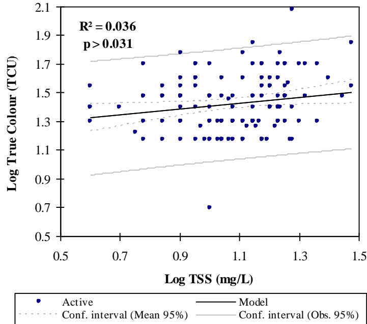
Figure 2H-39: Linear regression between total suspended solids (TSS) and true colour measured at sites located along the mainstem of the Nelson River: 2001–2004
