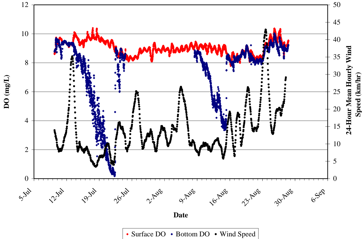
Figure 2H-25: Dissolved oxygen (DO) measured from loggers installed at Ross Wright Bay in Stephens Lake and 24-hour average hourly wind speed measured at Gillam: summer 2008
