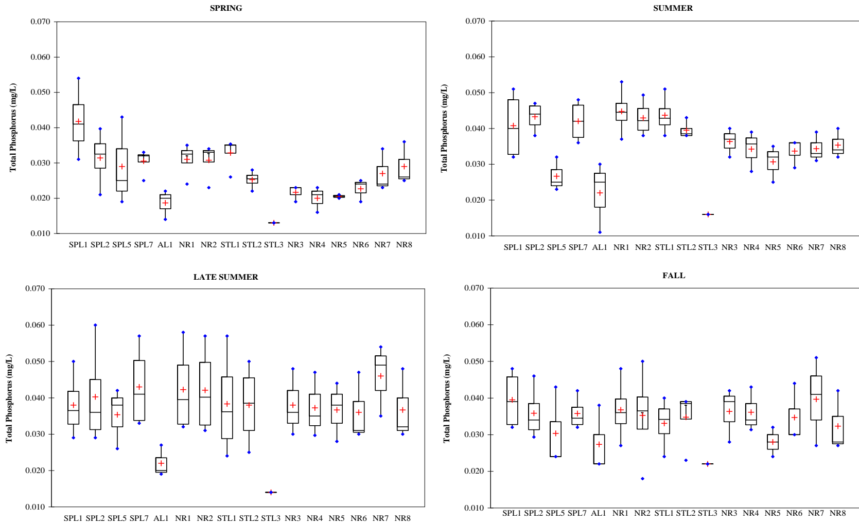
Figure 2H-1: Total phosphorus box plots for data collected from Split Lake to Gillam Island in the open water seasons 2001–2004. Data represent surface measurements
