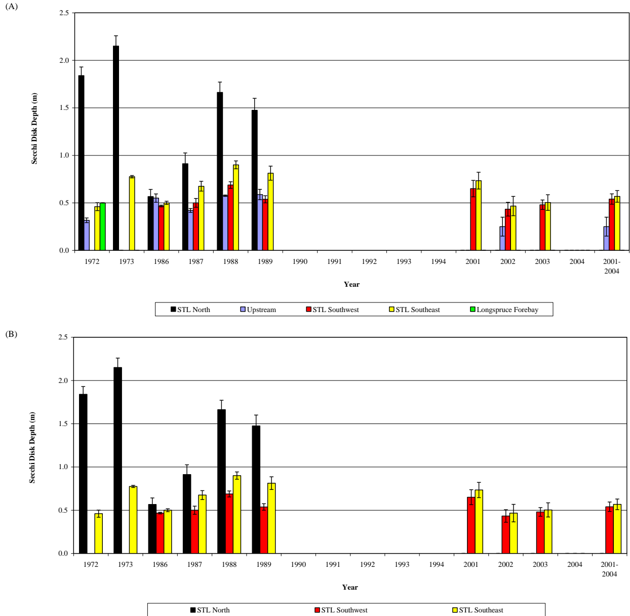
Figure 2E-1: Secchi disk depths (means ± standard error of the open water seasons) measured in Stephens Lake and upstream and downstream of the lake since 1972: (A) Stephens Lake and environs; and (B) Stephens Lake only
