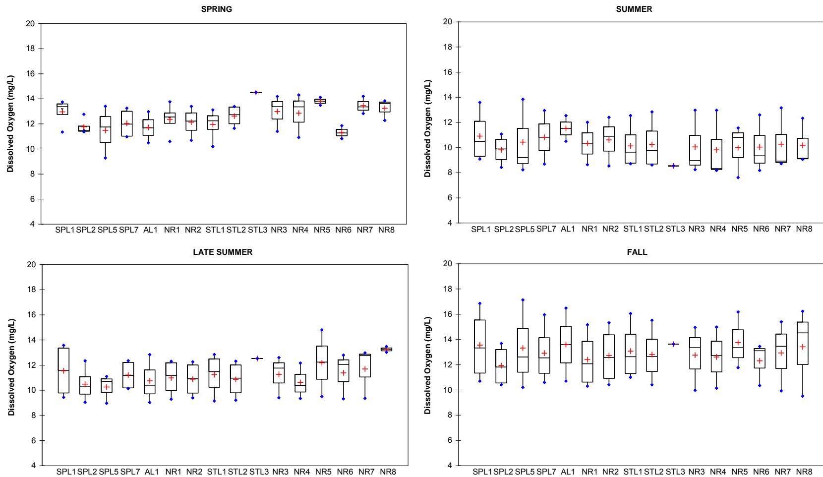
Figure 2H-3: Dissolved oxygen box plots for data collected from Split Lake to Gillam Island in the open water seasons 2001–2004. Data represent surface measurements
