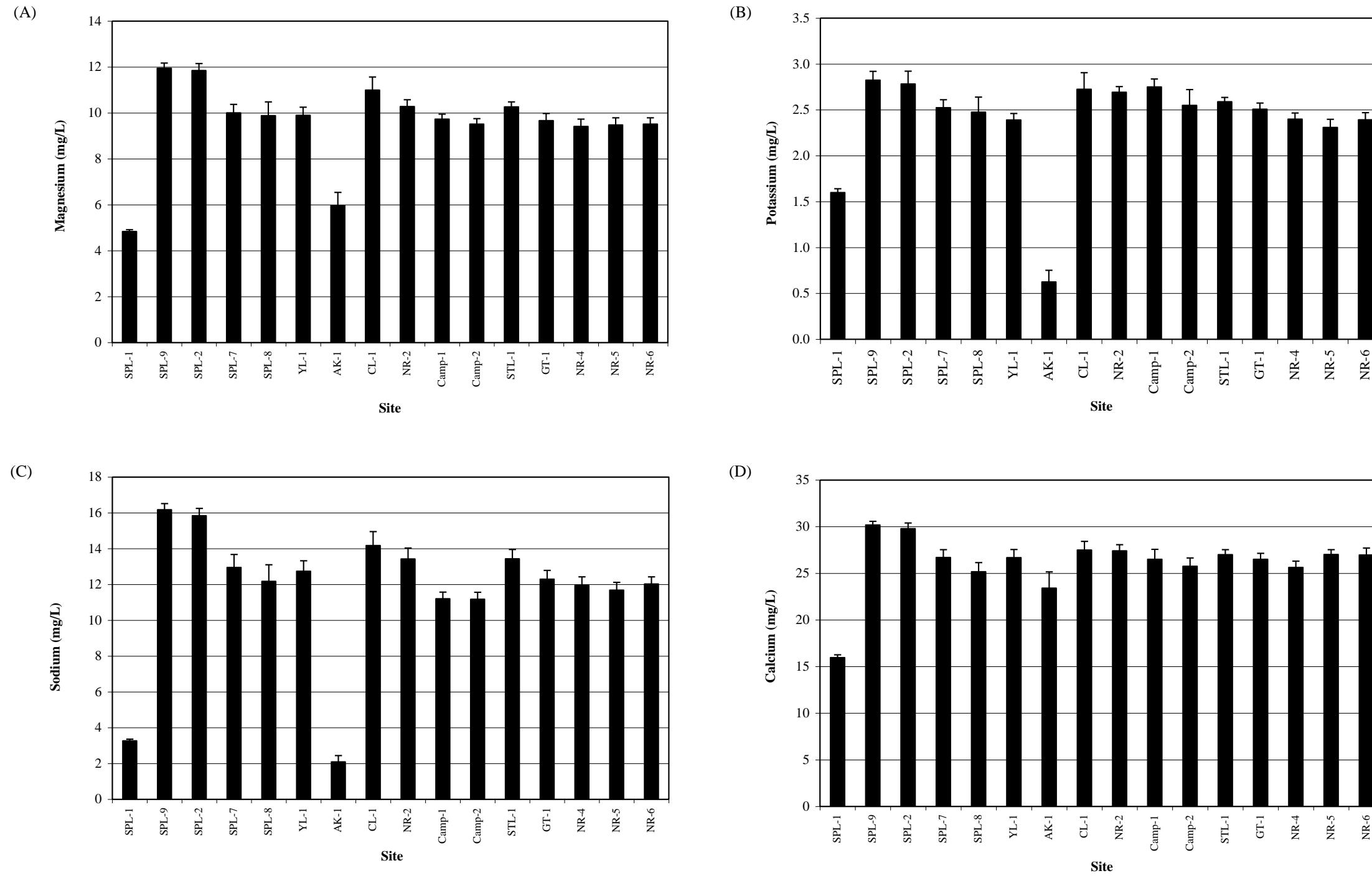
Figure 2-11: Open water season mean (±standard error) concentrations of (A) magnesium, (B) potassium, (C) sodium, and (D) calcium measured at sites in the Aquatic Environment Study Area: 2001–2004
