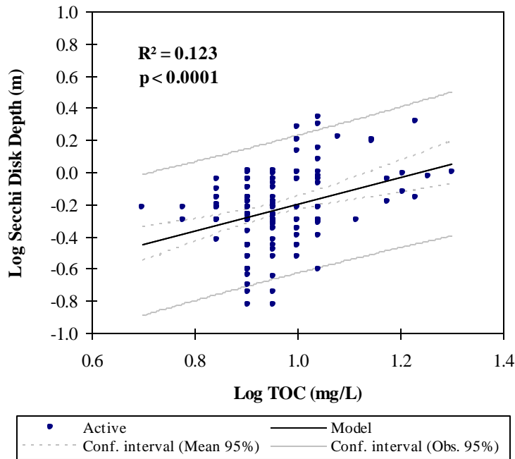
Figure 2H-32: Linear regression between total organic carbon (TOC) and Secchi disk depth measured across the study area: open water seasons 1999–2004
