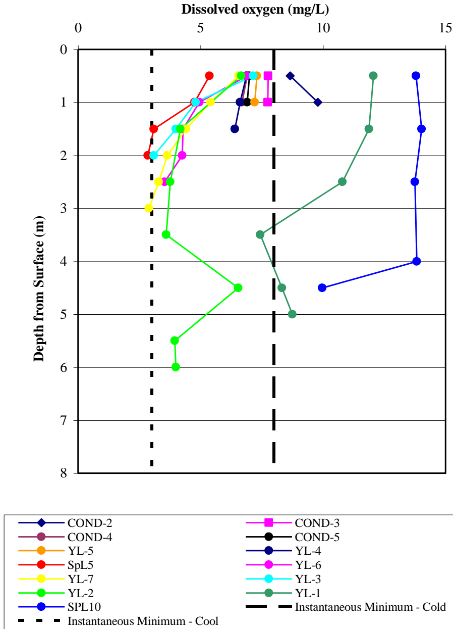
Figure 2H-15: Dissolved oxygen depth profiles measured in the York Landing area April 2007. Dashed lines represent the Manitoba instantaneous minimum DO objectives for the protection of cool-water and cold-water aquatic life
