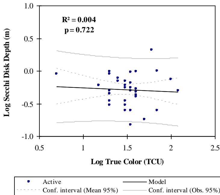
Figure 2H-33: Linear regression between true colour and Secchi disk depth measured across the study area: open water seasons 1999–2004
