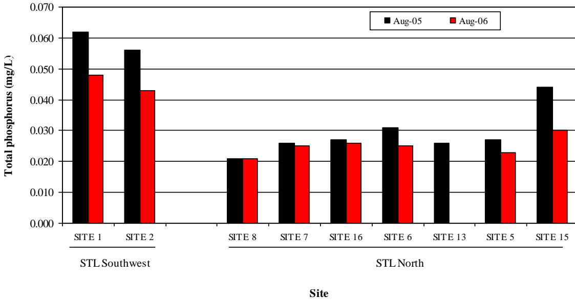
Figure 2H-36: Total phosphorus measured at sites located in the southwestern area of Stephens Lake (STL Southwest) and in the vicinity of O'Neil Bay (STL North). Sites in the north arm illustrated here represent a gradient from the nearshore area of O'Neil Bay out into the offshore area of the lake
