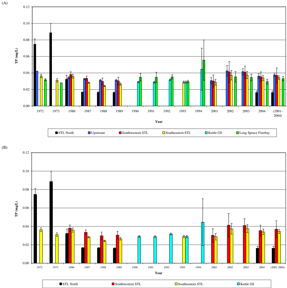
Figure 2E-2: Total phosphorus (TP) concentrations (means ± standard error of the open water seasons) measured in Stephens Lake and upstream and downstream of the lake since 1972: (A) Stephens Lake and environs; and (B) Stephens Lake only
