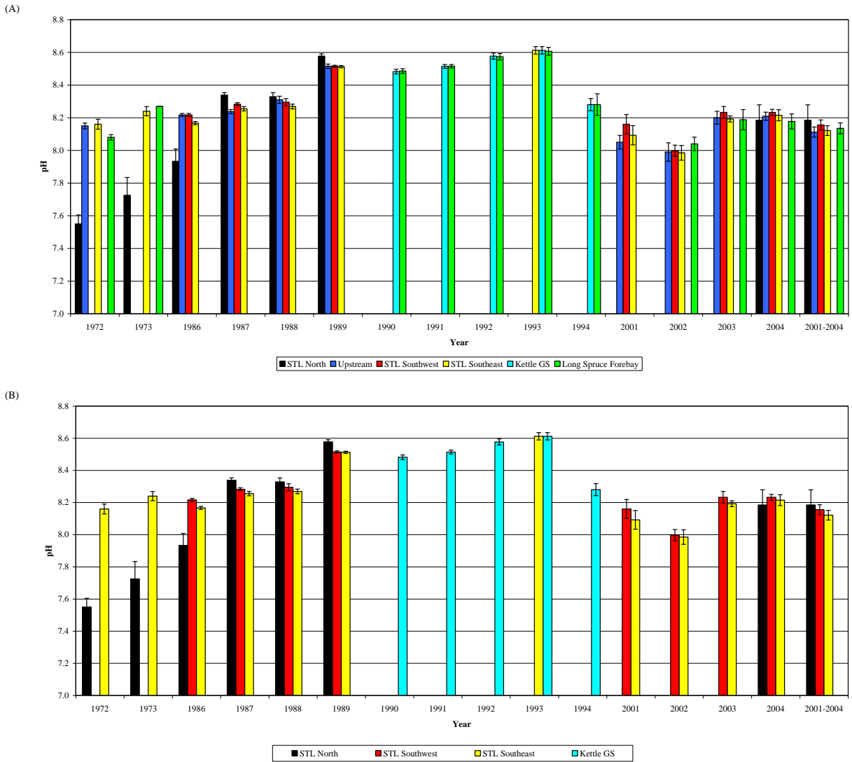
Figure 2E-6: Laboratory pH (means \pm standard error of the open water seasons) measured in Stephens Lake and upstream and downstream of the lake since 1972: (A) Stephens Lake and environs; and (B) Stephens Lake only
