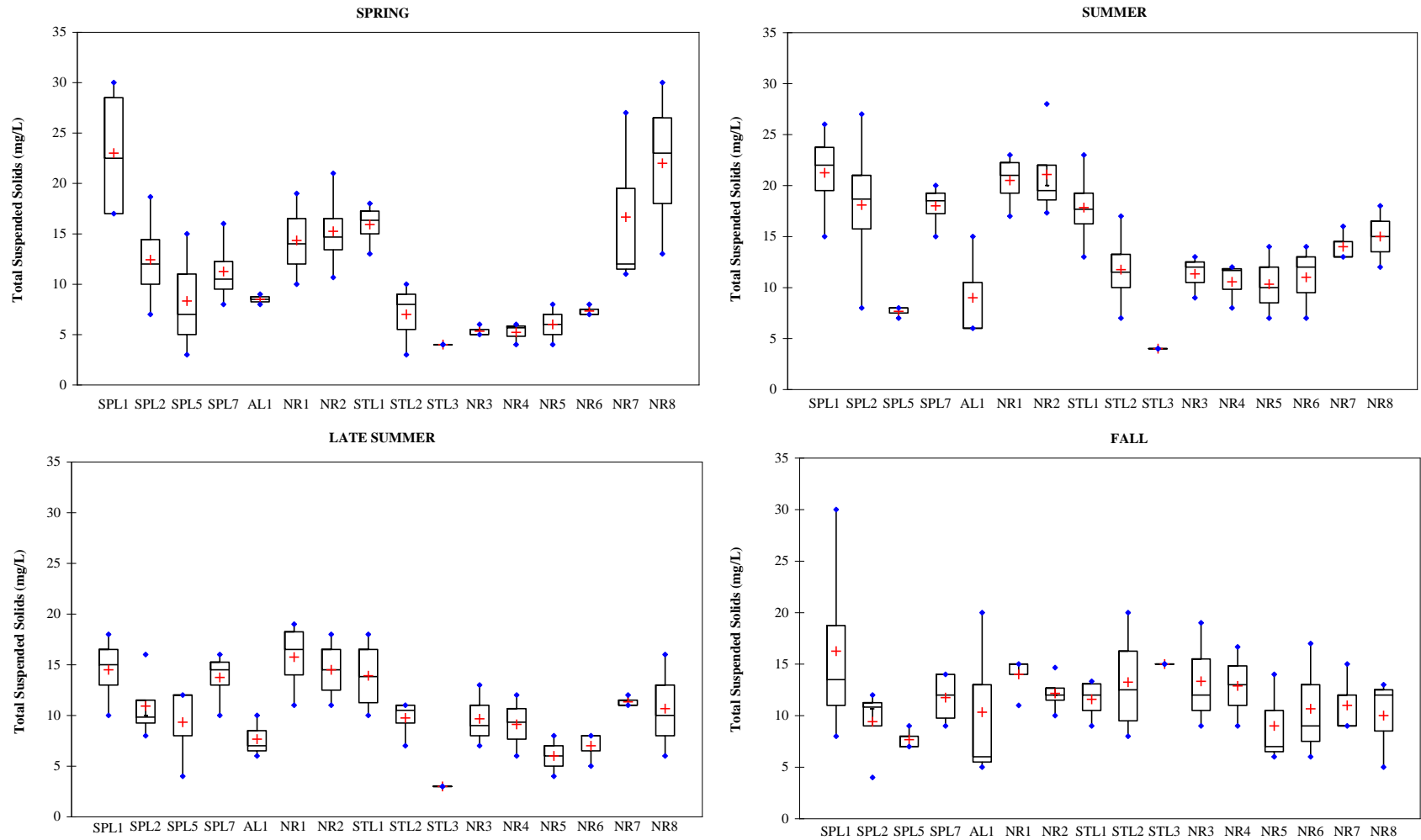
Figure 2H-7: Total suspended solids box plots for data collected from Split Lake to Gillam Island in the open water seasons 2001–2004. Data represent surface measurements
