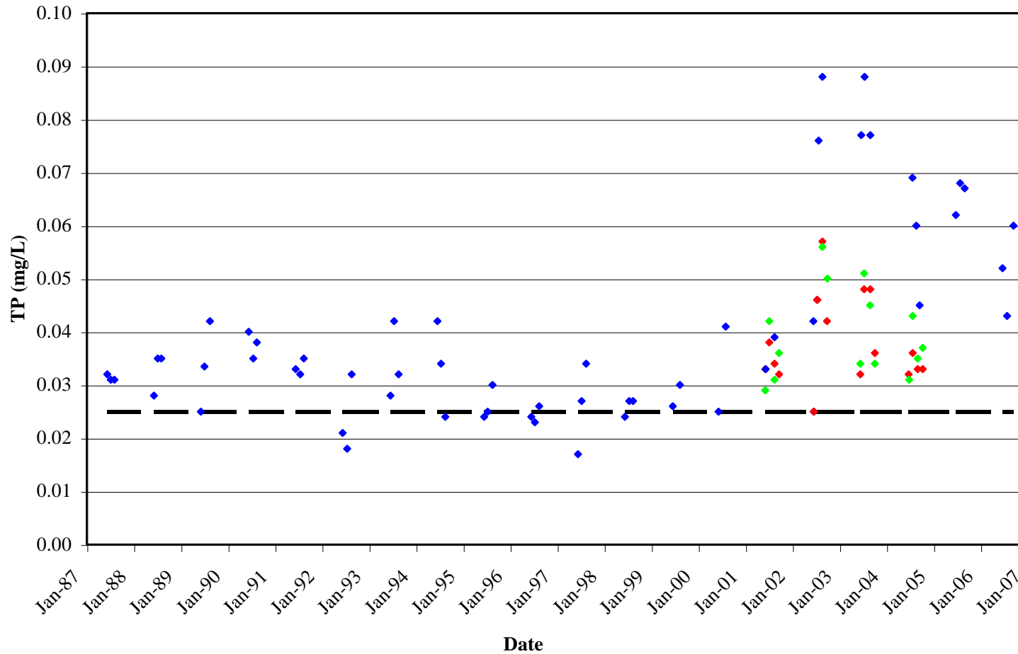
Figure 2D-1: Comparison of total phosphorus (TP) concentrations measured in Split Lake by Manitoba Water Stewardship (blue dots) and under the Keyask environmental studies (red dots SPL7 and green dots SPL8) for the open water season. The dashed line indicates the Manitoba Water Quality Standards, Objectives, and Guidelines (MWQSOG) for lakes, ponds, and reservoirs
