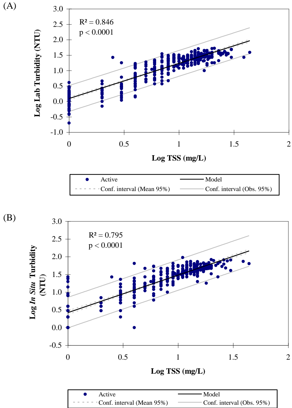
Figure 2H-22: Linear regression between lab turbidity and total suspended solids (TSS) (A) and in situ turbidity and TSS (B) measured across the study area: open water seasons 1999–2004
