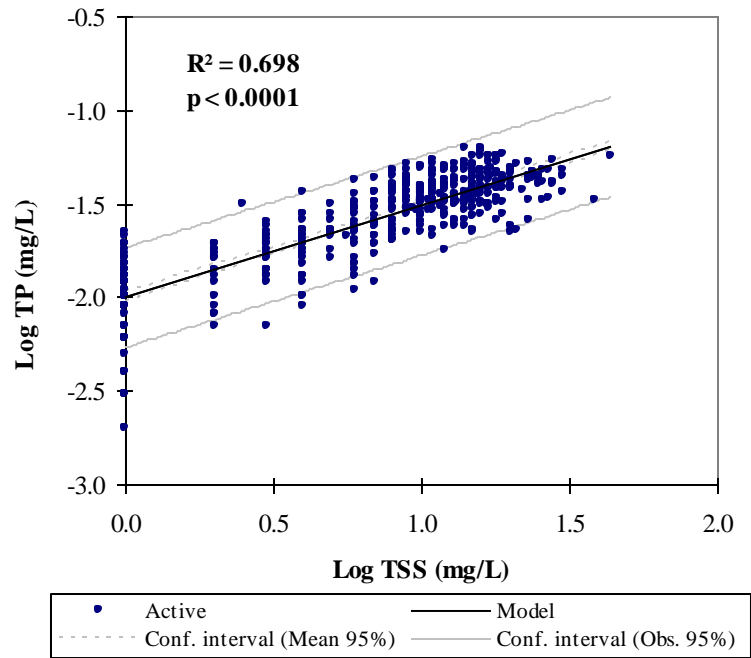
Figure 2H-8: Linear regression between total phosphorus (TP) and total suspended solids (TSS) measured across the study area: open water seasons 1999–2004. Regressions should be interpreted with caution; data did not meet the assumptions of normality
