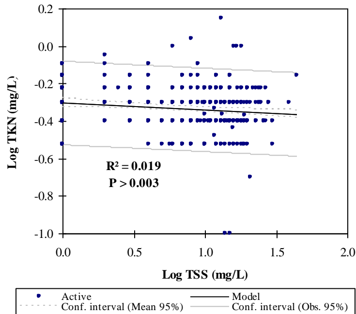
Figure 2H-41: Linear regression between total suspended solids (TSS) and total Kjeldahl nitrogen (TKN) measured across the study area: 2001–2004
