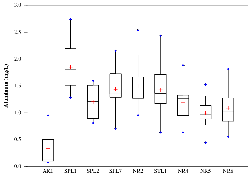
Figure 2H-11: Total aluminum box plots for data collected from the study area in the open water seasons 2001–2004. Data represent surface measurements. Dashed line indicates the Manitoba and Canadian Council of Ministers of the Environment water quality guideline for the protection of aquatic life
