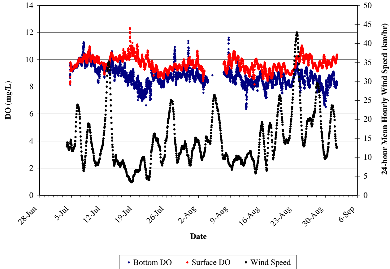
Figure 2H-20: Dissolved oxygen (DO) measured from loggers installed at John Garson Bay along the Nelson River and 24-hour average hourly wind speed measured at Gillam: summer 2008
