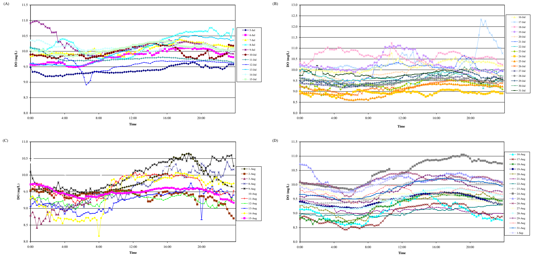
Figure 2H-19: Dissolved oxygen (DO) data collected from near the water surface in John Garson Bay illustrating diurnal changes: (A) 5–15 July; (B) 16–31 July; (C) 1–15 August; and (D) 16 August to 1 September 2008
