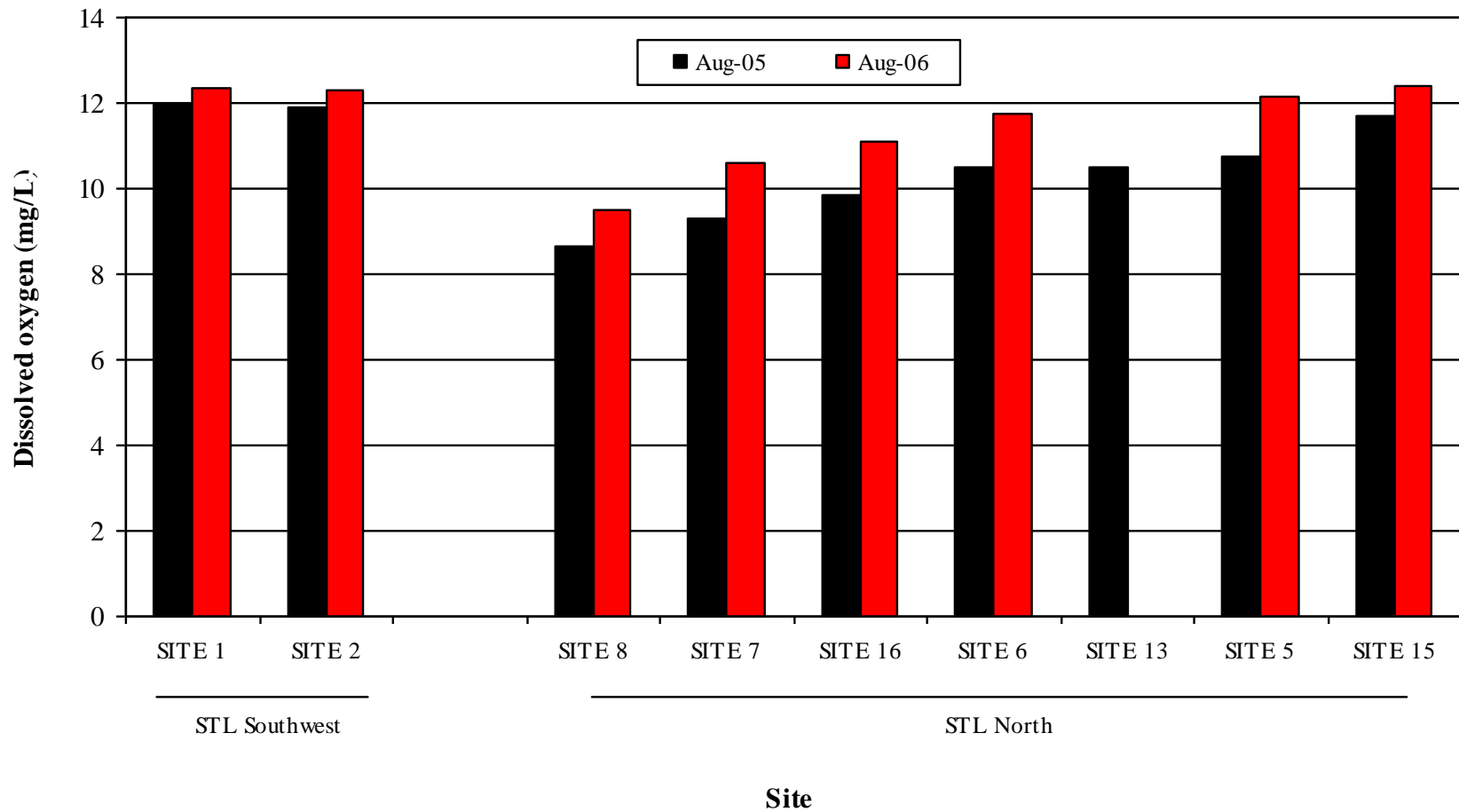
Figure 2H23: Dissolved oxygen concentrations measured at sites located in the southwestern area of Stephens Lake (STL Southwest) and in the vicinity of O'Neil Bay (STL North). Sites in the north arm illustrated here represent a gradient from the nearshore area of O'Neil Bay out into the offshore area of the lake
