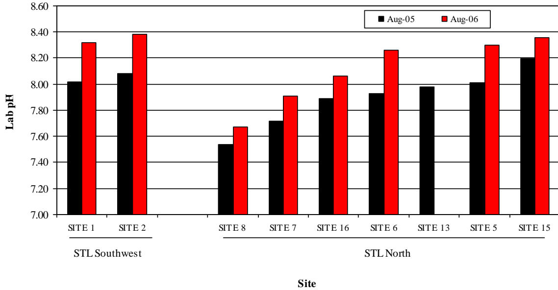
Figure 2H-34: pH measured at sites located in the southwestern area of Stephens Lake (STL Southwest) and in the vicinity of O'Neil Bay (STL North). Sites in the north arm illustrated here represent a gradient from the nearshore area of O'Neil Bay out into the offshore area of the lake
