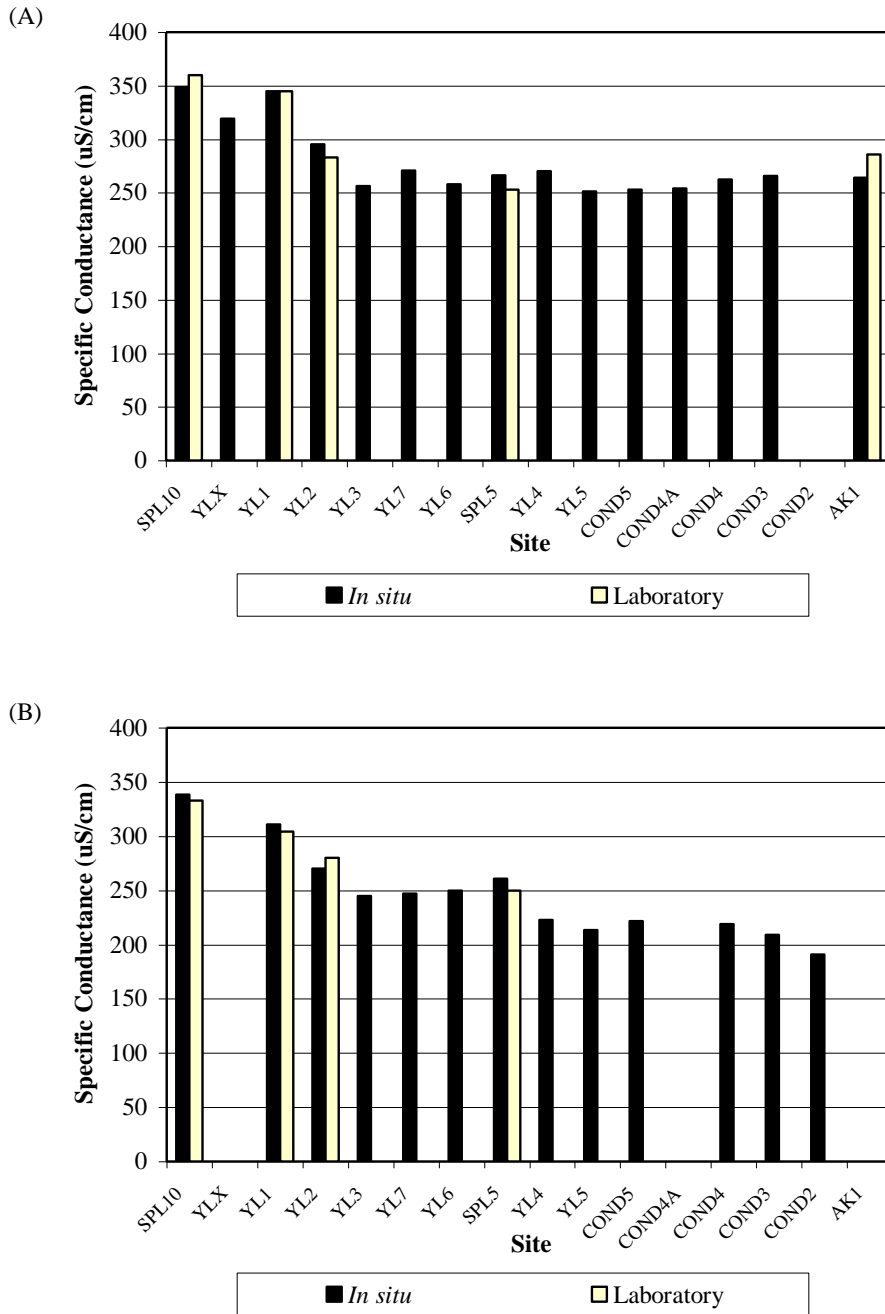
Figure 2H-17: Specific conductance measured in the York Landing area: (A) February 2007; and (B) April 2007. Values illustrated represent mean (depth-averaged) in situ and laboratory measurements. Samples of surface water were collected for laboratory analysis at sites SPL10, YL1, YL2, SPL5, and AK1 in February and SPL10, YL1, YL2, and SPL5 in April
