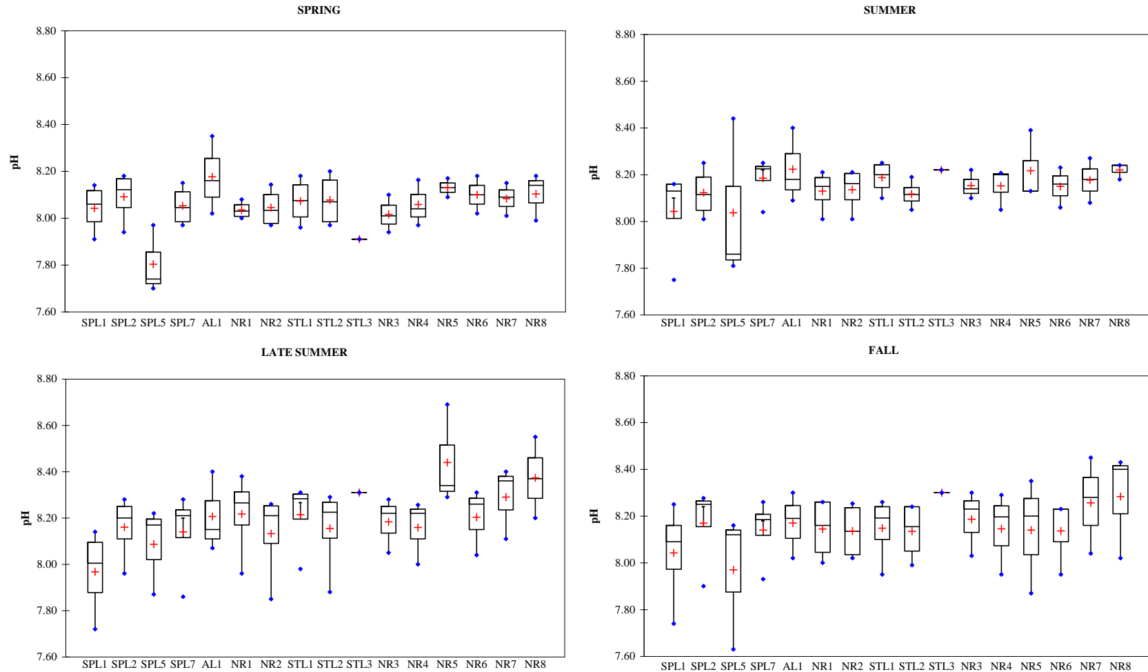
Figure 2H-4: pH (laboratory) box plots for data collected from Split Lake to Gillam Island in the open water seasons 2001–2004. Data represent surface measurements
