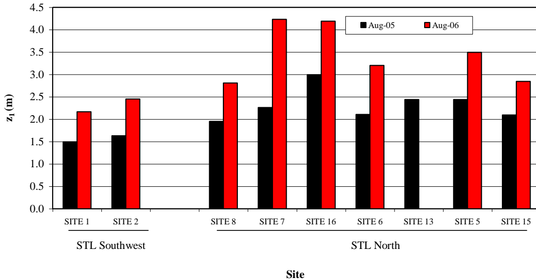
Figure 2H-29: Euphotic zone depth (z 1 ) measured at sites located in the southwestern area of Stephens Lake (STL Southwest) and in the vicinity of O'Neil Bay (STL North). Sites in the north arm illustrated here represent a gradient from the nearshore area of O'Neil Bay out into the offshore area of the lake
