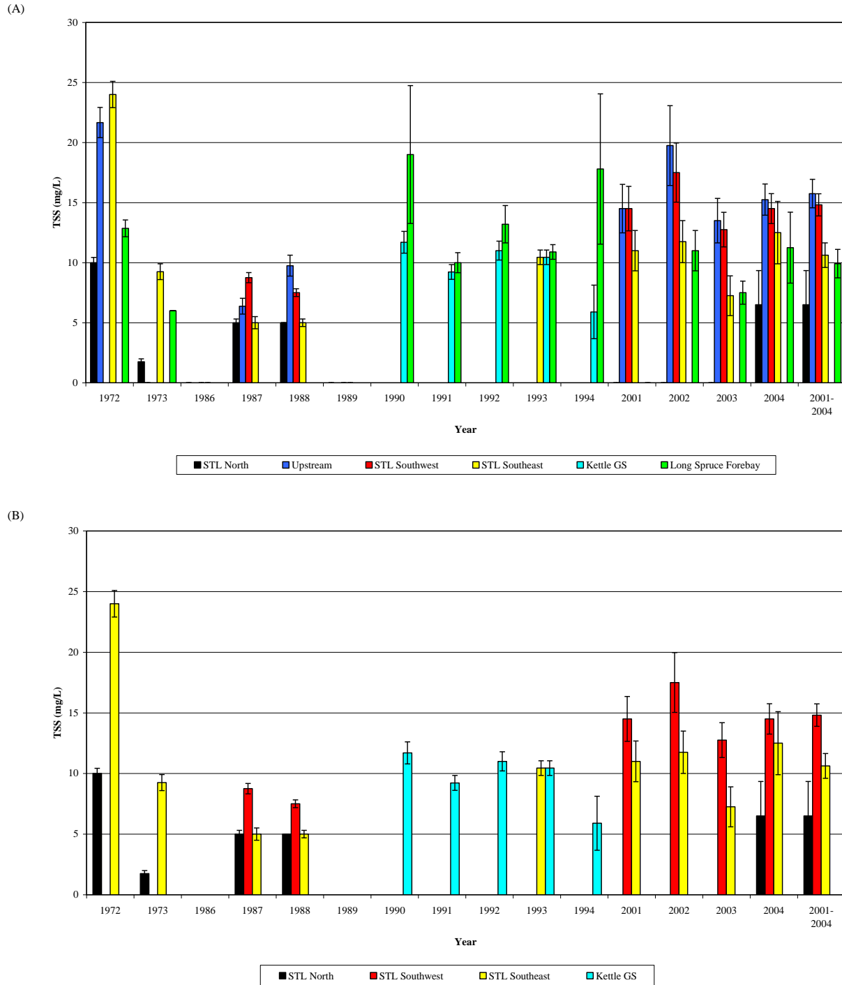
Figure 2E-9: Total suspended solids (means ± standard error of the open water seasons) measured in Stephens Lake and upstream and downstream of the lake since 1972: (A) Stephens Lake and environs; and (B) Stephens Lake only
