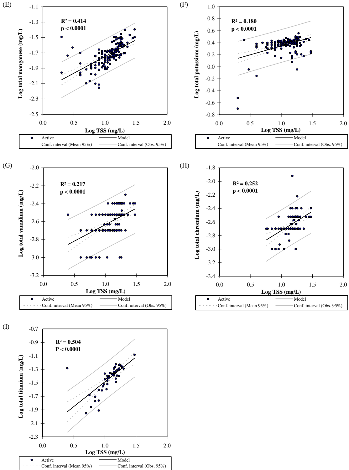
Figure 2H-14: Linear regression between total suspended solids (TSS) and (A) iron, (B) aluminum, (C) barium, (D) cobalt, (E) manganese, (F) potassium, (G) vanadium, (H) chromium, and (I) titanium measured across the study area: open water seasons 1999–2004
