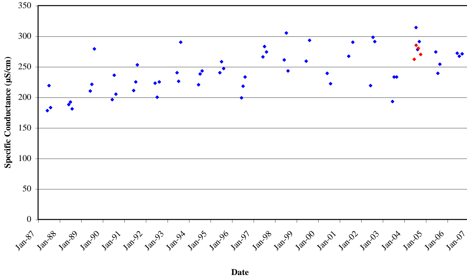
Figure 2D-7: Comparison of specific conductance (laboratory) measured in Split Lake by Manitoba Water Stewardship (blue dots) and under the Keyyask environmental studies (red dots SPL7) for the open water season
