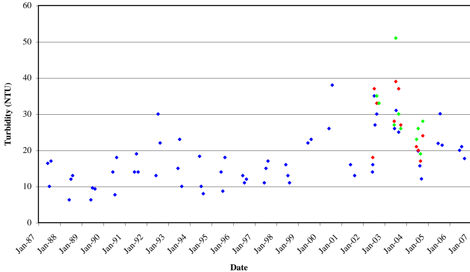
Figure 2D-4: Comparison of turbidity measured in Split Lake by Manitoba Water Stewardship (blue dots) and under the Keyask environmental studies (red dots SPL7 and green dots SPL8) for the open water season
