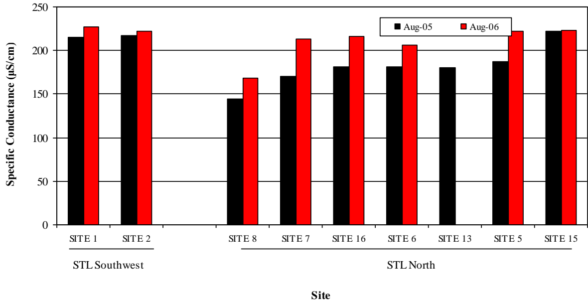
Figure 2H-35: Specific conductance measured at sites located in the southwestern area of Stephens Lake (STL Southwest) and in the vicinity of O'Neil Bay (STL North). Sites in the north arm illustrated here represent a gradient from the nearshore area of O'Neil Bay out into the offshore area of the lake
