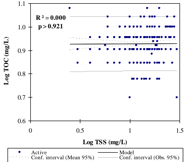
Figure 2H-40: Linear regression between total suspended solids (TSS) and total organic carbon (TOC) measured at sites located along the mainstem of the Nelson River: 2001–2004
