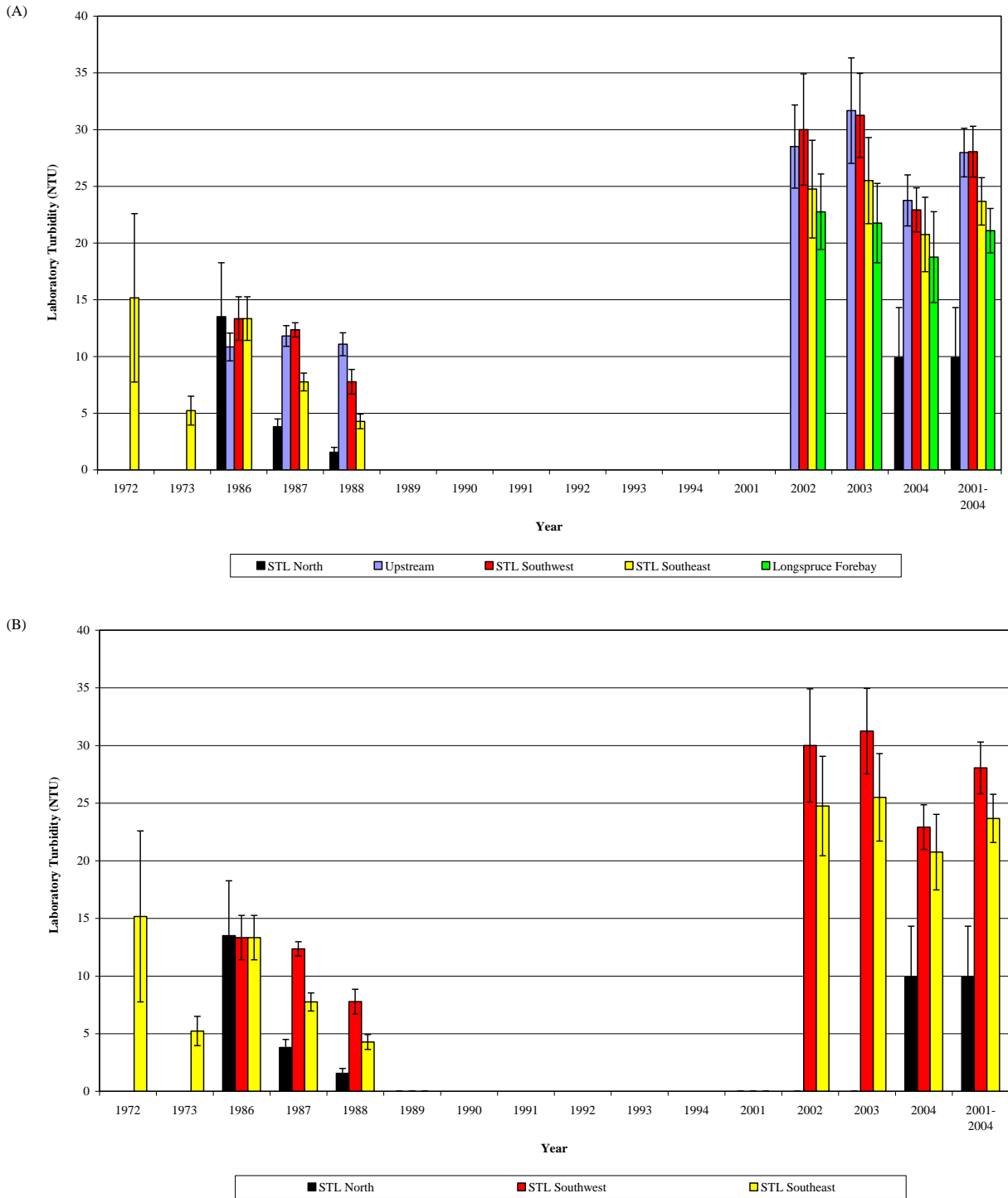
Figure 2E-8: Laboratory turbidity (means ± standard error of the open water seasons) measured in Stephens Lake and upstream and downstream of the lake since 1972: (A) Stephens Lake and environs; and (B) Stephens Lake only
