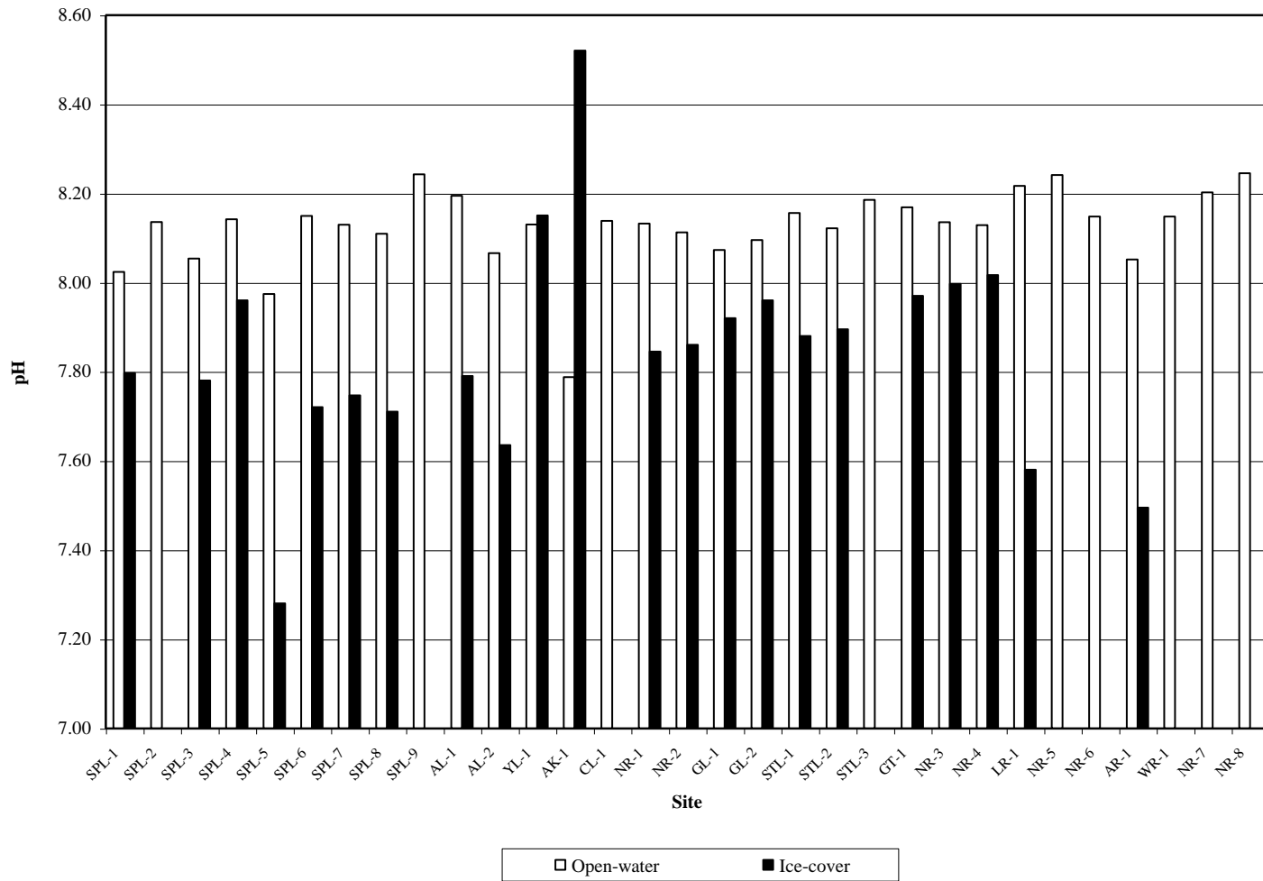
Figure 2H-16: Comparison of mean pH (laboratory) values measured in the open water and ice-cover seasons in the study area 2001–2007
