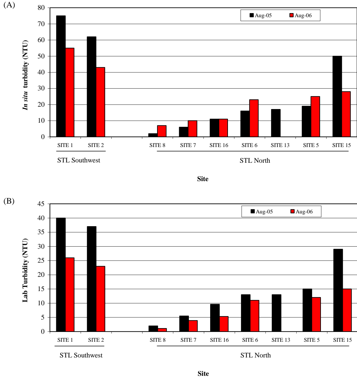
Figure 2H-27: Turbidity ((A) in situ and (B) laboratory) measured at sites located in the southwestern area of Stephens Lake (STL Southwest) and in the vicinity of O’Neil Bay (STL North). Sites in the north arm illustrated here represent a gradient from the nearshore area of O’Neil Bay out into the offshore area of the lake
