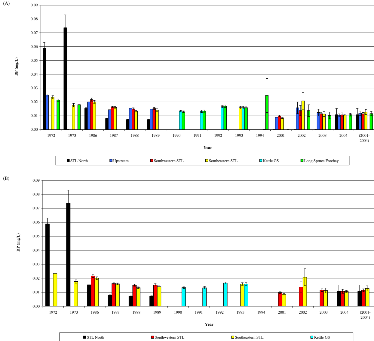
Figure 2E-3: Total dissolved phosphorus (DP) concentrations (means ± standard error of the open water seasons) measured in Stephens Lake and upstream and downstream of the lake since 1972: (A) Stephens Lake and environs; and (B) Stephens Lake only
