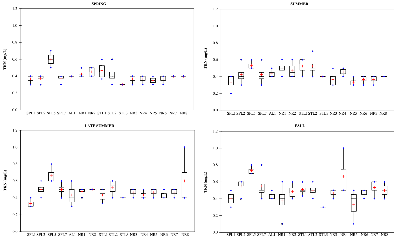
Figure 2H-2: Total Kjeldahl nitrogen (TKN) box plots for data collected from Split Lake to Gillam Island in the open water seasons 2001–2004. Data represent surface measurements
