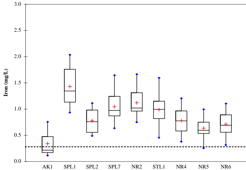
Figure 2H-10: Total iron box plots for data collected in the study area in the open water seasons 2001–2004. Data represent surface measurements. Dashed line indicates the Manitoba and Canadian Council of Ministers of the Environment water quality guideline for the protection of aquatic life and the aesthetic drinking water quality guideline
