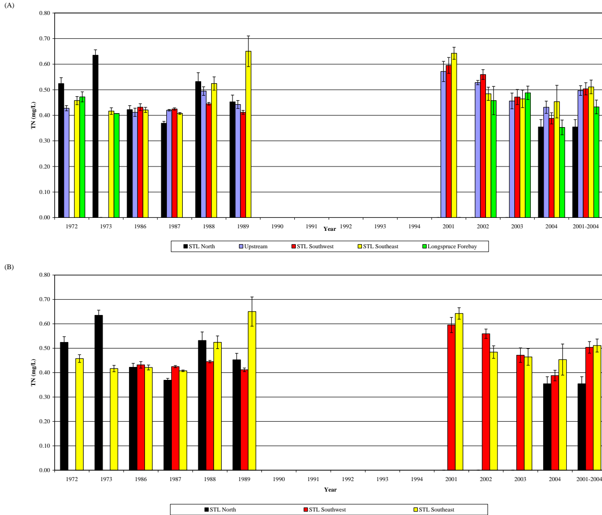
Figure 2E-5: Total nitrogen (means ± standard error of the open water seasons) measured in Stephens Lake and upstream and downstream of the lake since 1972: (A) Stephens Lake and environs; and (B) Stephens Lake only
