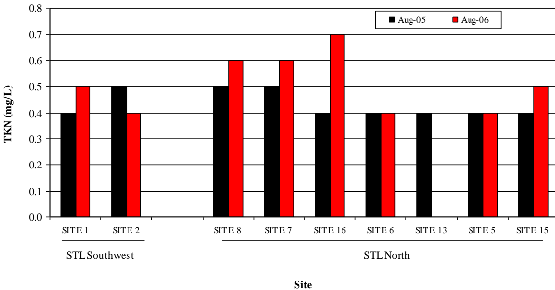
Figure 2H-37: Total Kjeldahl nitrogen (TKN) measured at sites located in the southwestern area of Stephens Lake (STL Southwest) and in the vicinity of O'Neil Bay (STL North). Sites in the north arm illustrated here represent a gradient from the nearshore area of O'Neil Bay out into the offshore area of the lake
