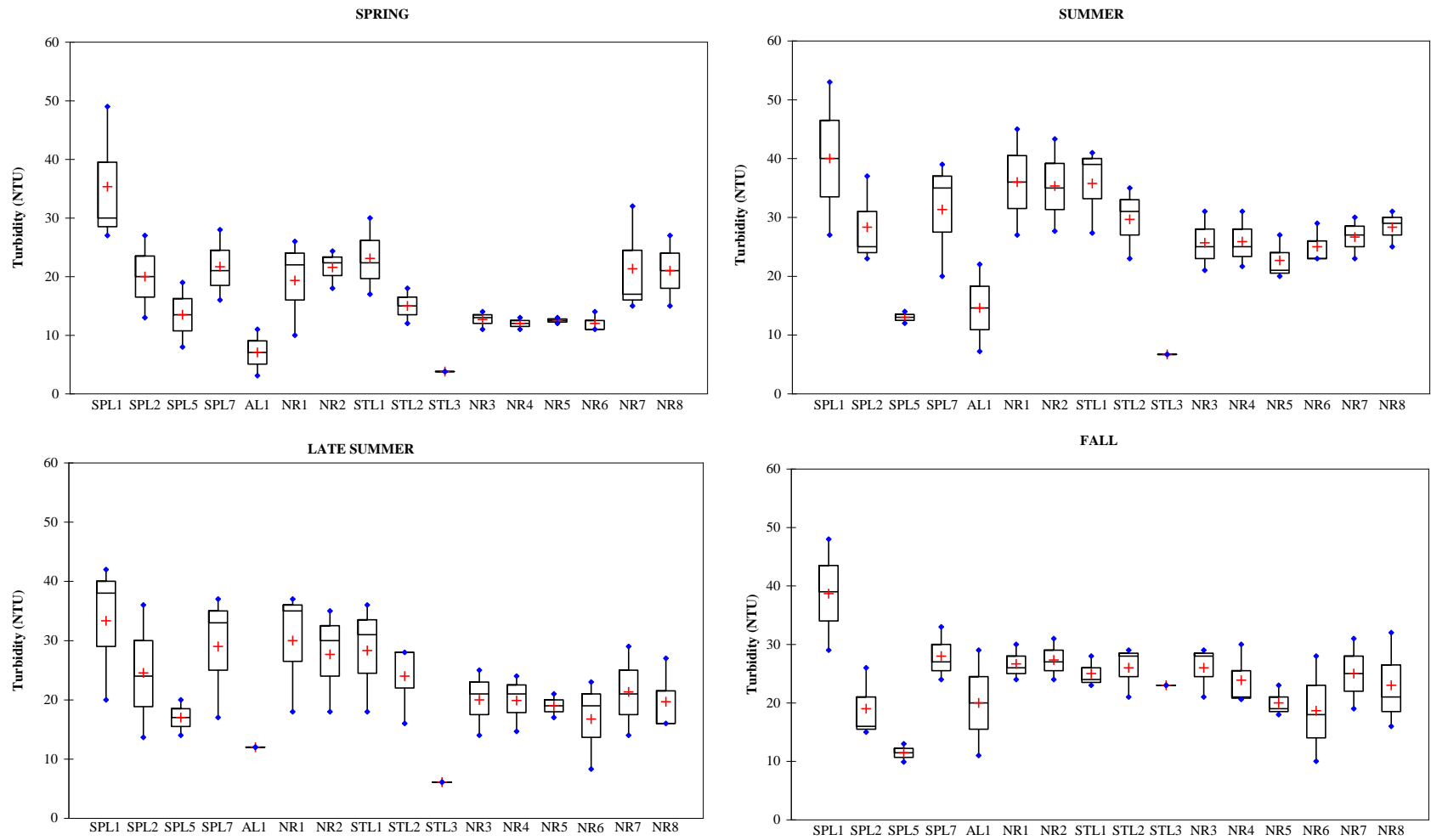
Figure 2H-5: Turbidity (laboratory) box plots for data collected from Split Lake to Gillam Island in the open water seasons 2001–2004. Data represent surface measurements
