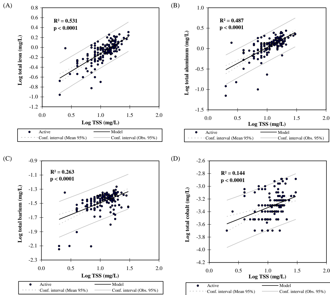
Figure 2H-14: Linear regression between total suspended solids (TSS) and (A) iron, (B) aluminum, (C) barium, (D) cobalt, (E) manganese, (F) potassium, (G) vanadium, (H) chromium, and (I) titanium measured across the study area: open water seasons 1999–2004
